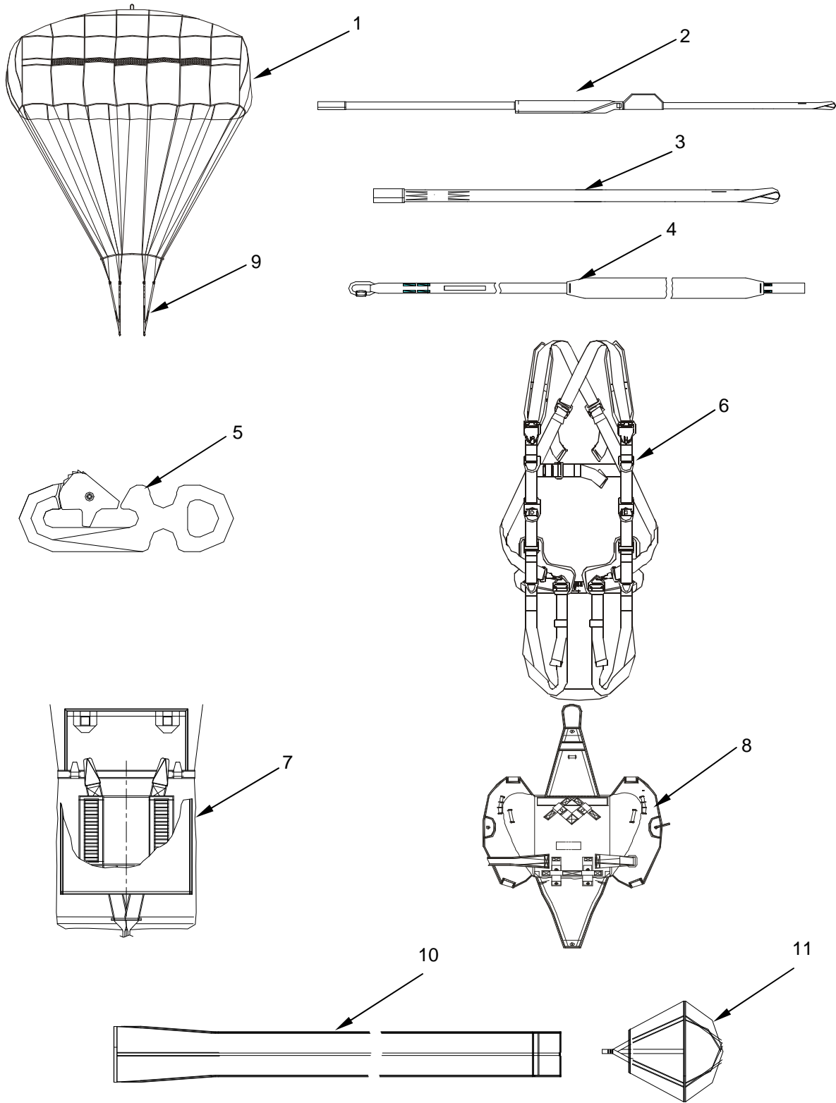
Figure 1. T-11 Personnel Parachute System (Sheet 1 of 2).
