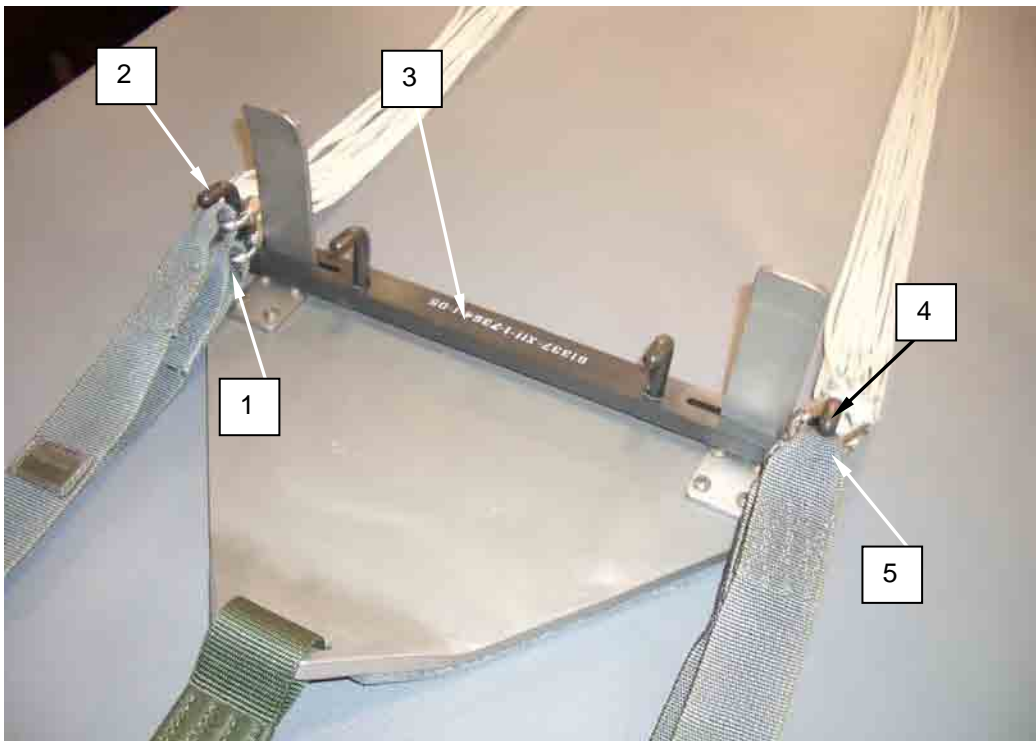
Figure 1. Place Connector Links on Tension Plate Adapter.
