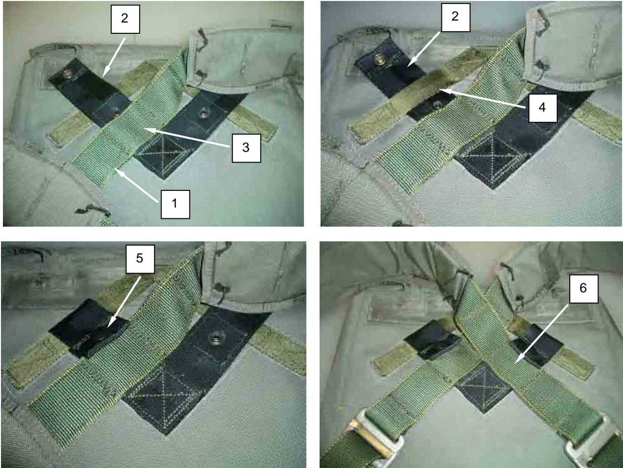
Figure 6. Route Diagonal Back Strap Keeper.
