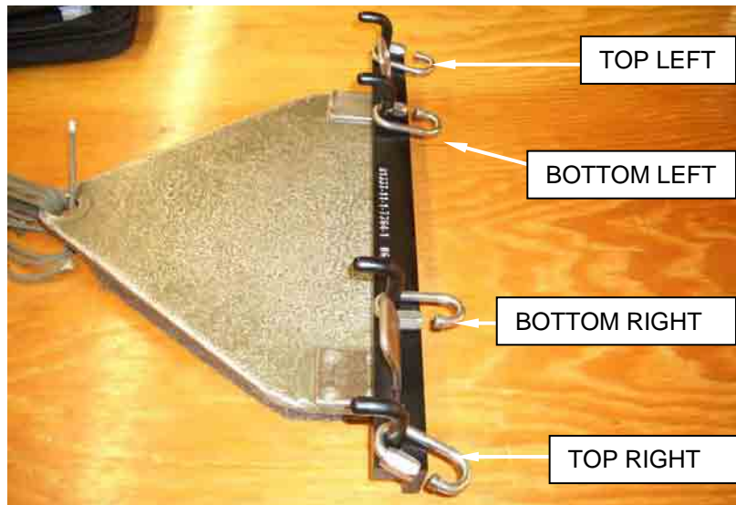
Figure 2. Tension Plate Adapter Layout.
