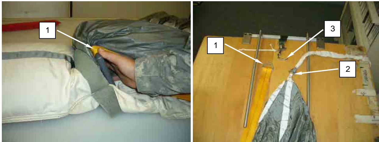
Figure 31. Release Packing Loop Tension Device.
