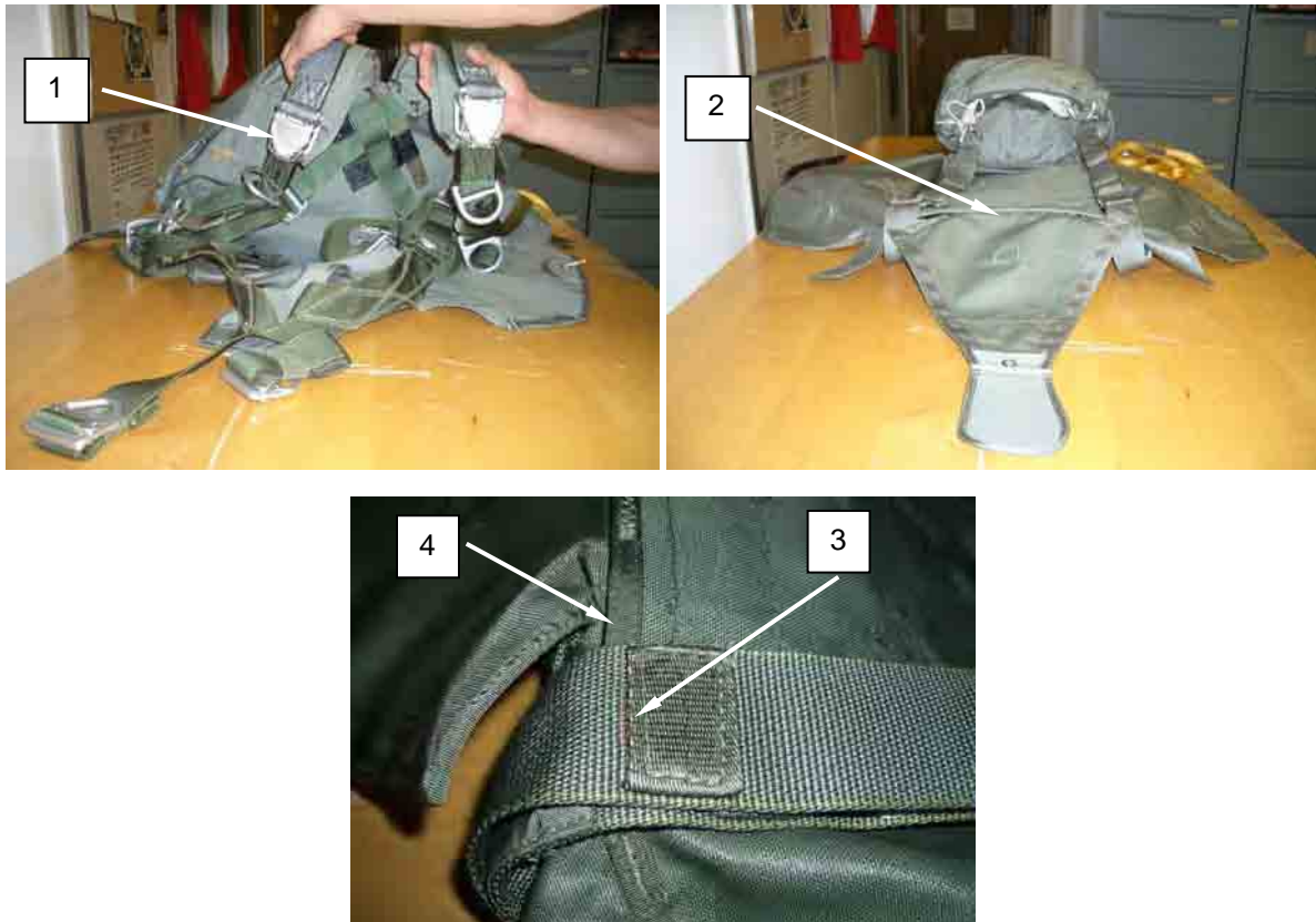
Figure 54. Rotate Main Pack Tray under Risers.
