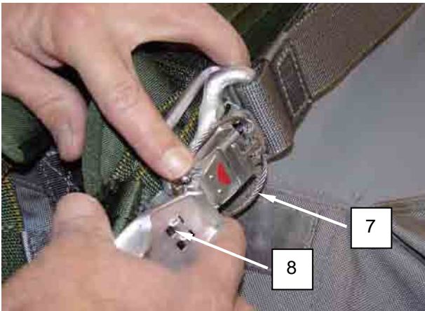
Figure 18. Laying Out Risers and Harness Assembly, and Assembling Risers and Harness Assembly.
