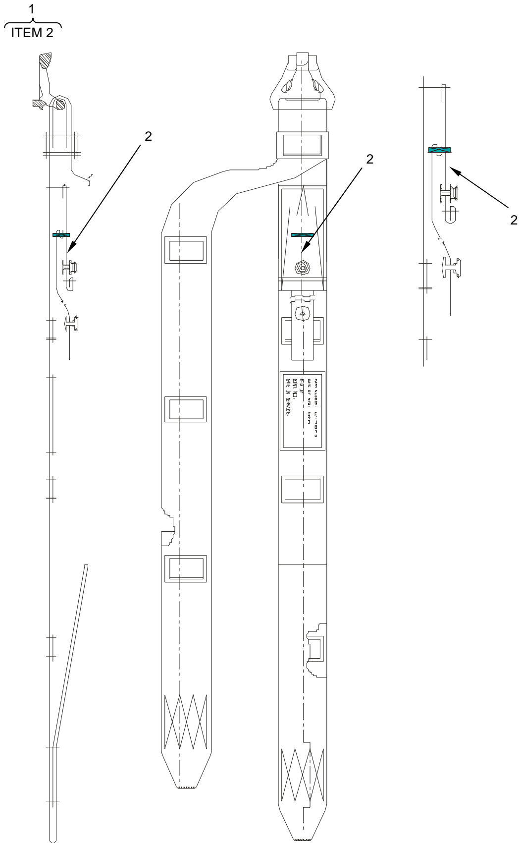
Figure 3. T-11 Main Riser Set.
