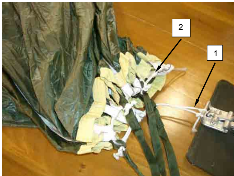
Figure 1. Passing Apex Hook Lanyard through All Apex Loops.
