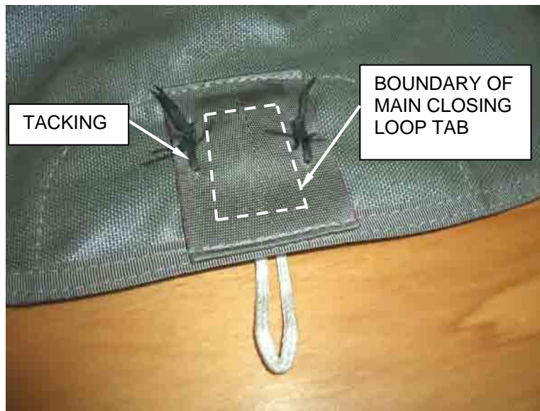
Figure 4. Tacking Both Sides of the Protective Cover.
