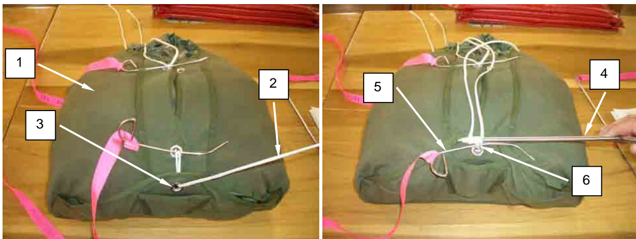
Figure 56. Using T-bar To Close Pack Tray and Inserting Temporary Pin.
