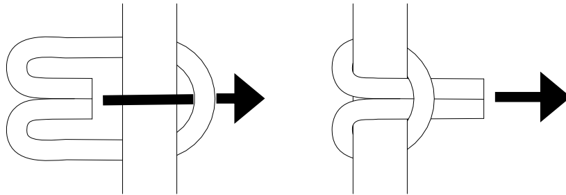
Figure 22. Girth Hitch.
