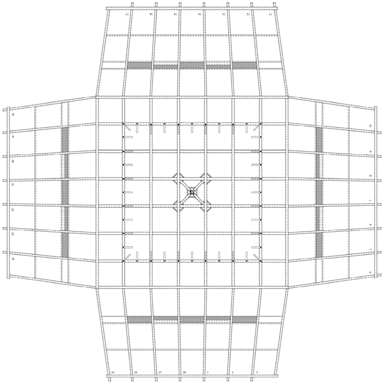
Figure 26. T-11 Main Canopy.
