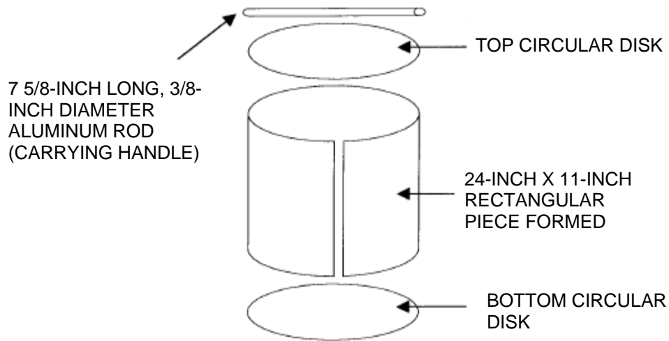
Figure 3. Fabricating 32 Pound Weight.
