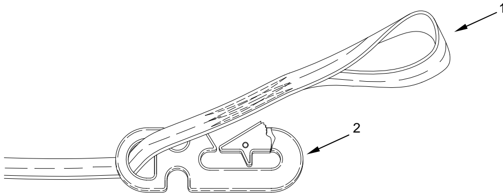
Figure 3. Pass Loop End of Static Line or Static Line Extension through Opening in Base of Snap Hook.
