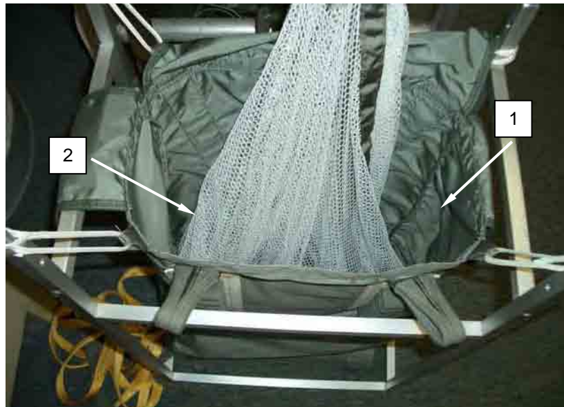
Figure 40. Place Drogue Parachute in Bottom of Deployment Bag.
