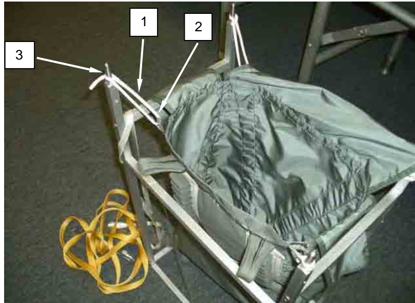
Figure 39. Secure Deployment Bag to Deployment Cradle.
