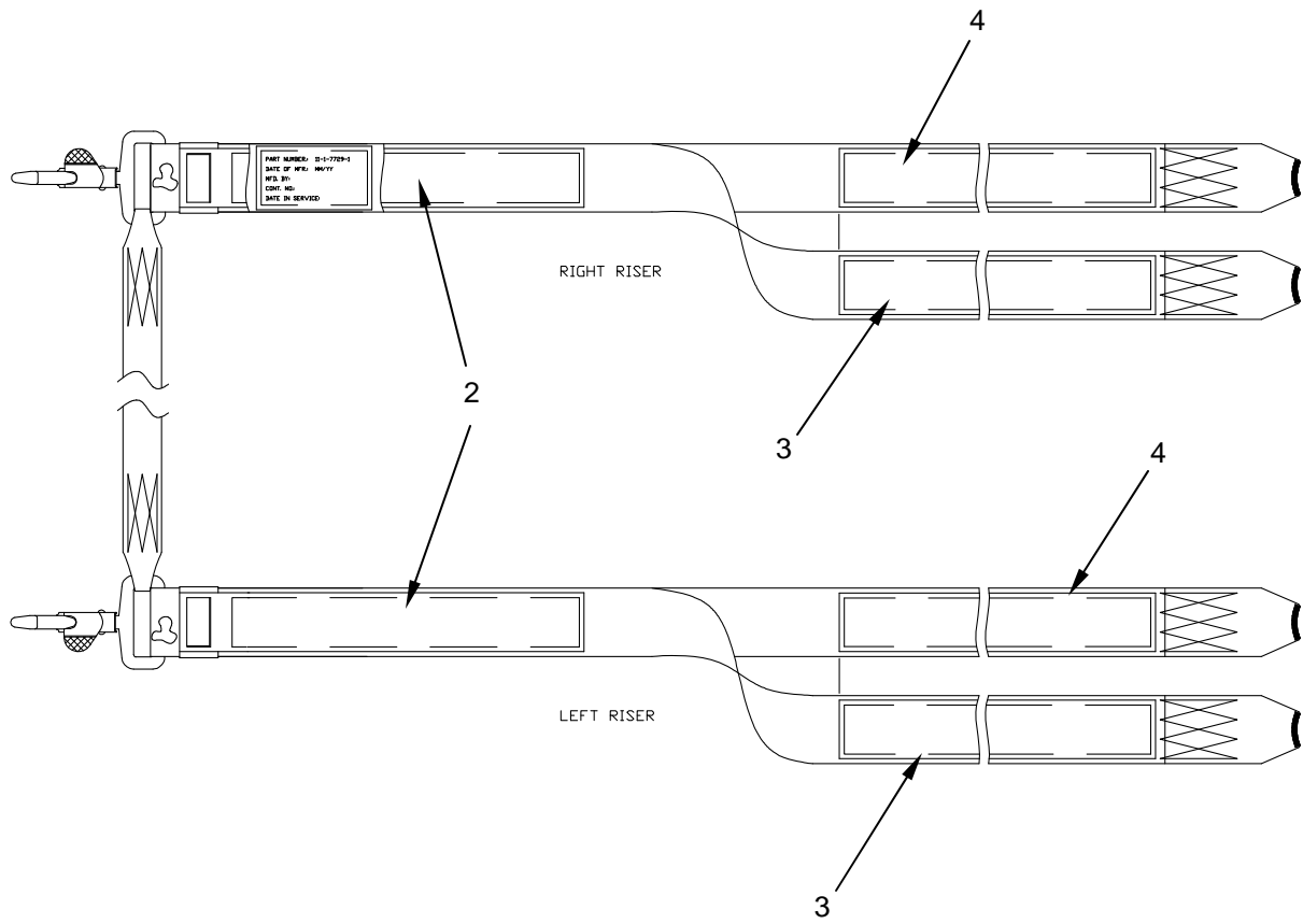
Figure 7. T-11 Reserve Riser Set.
