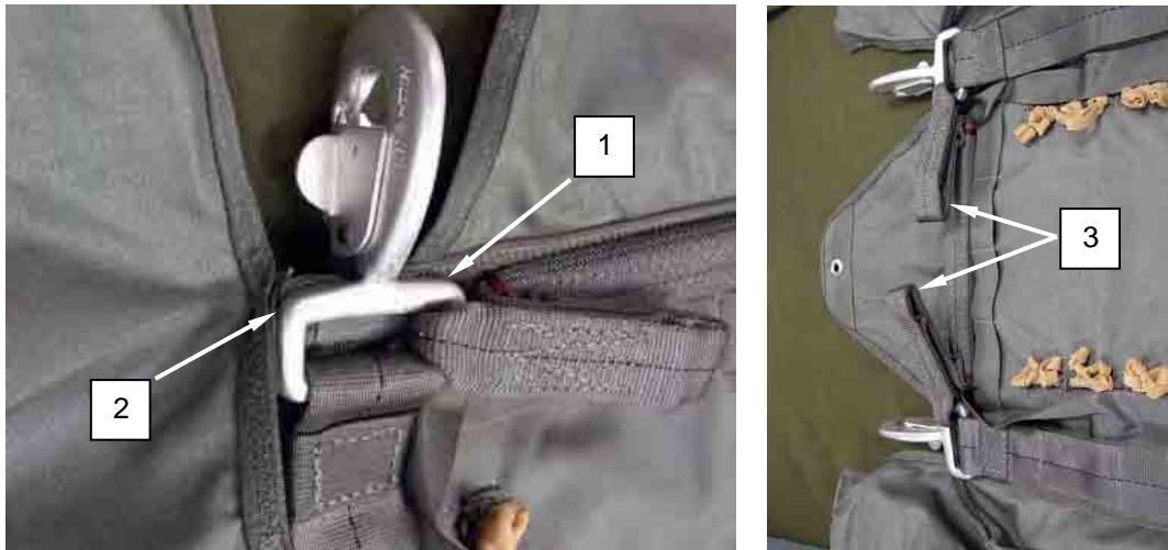
Figure 2. Aligning Top Bar of Snap Hook with Binding Tape and S-Folding Excess Spreader Bar.
