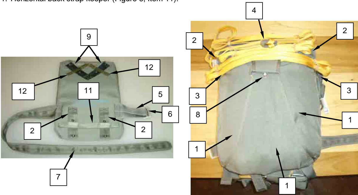
Figure 6. Main Pack Tray.
