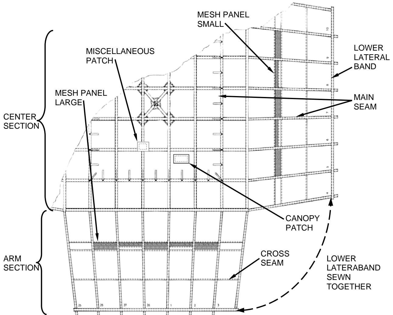
Figure 6. Canopy Layout and Patch Construction.
