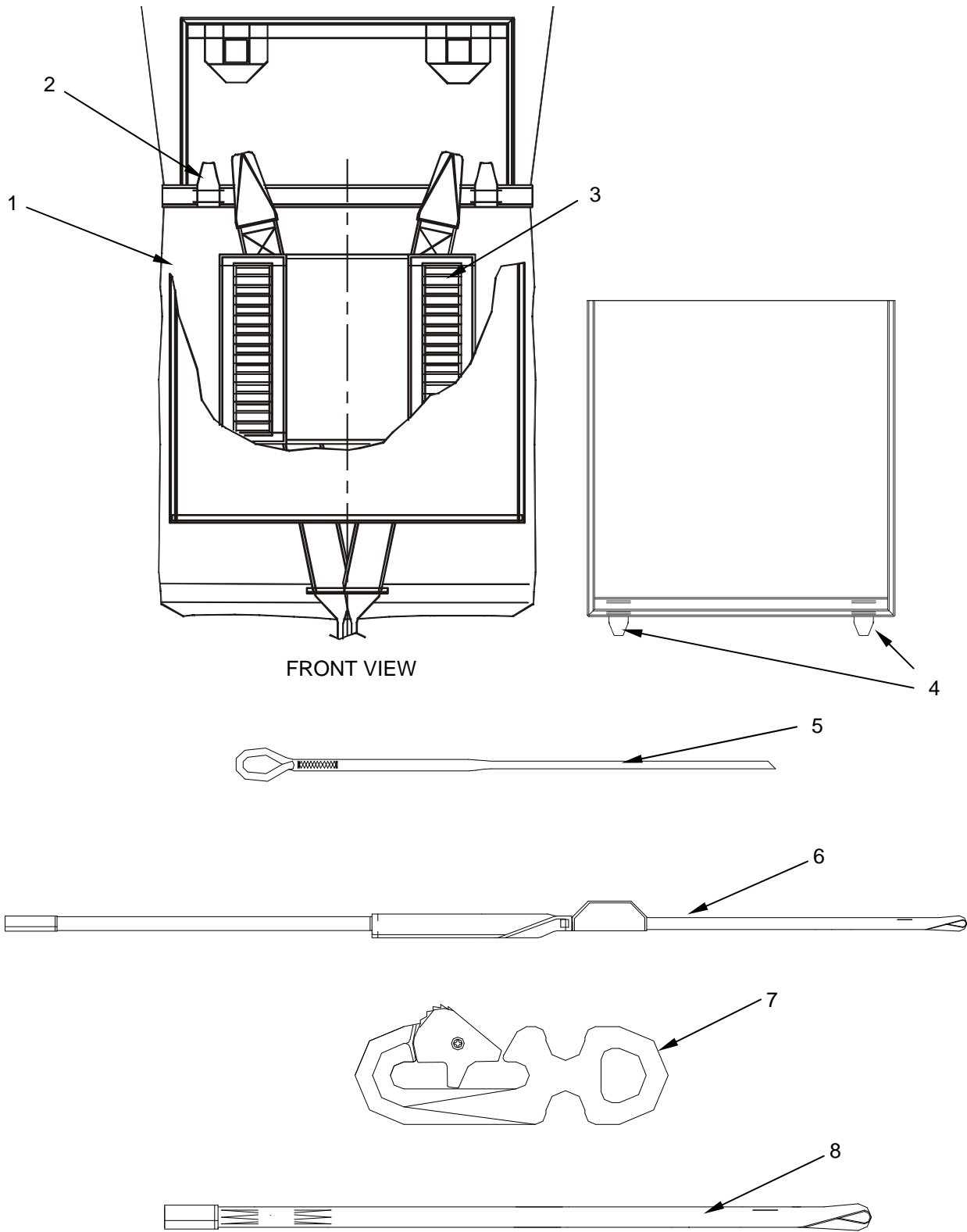
Figure 9. T-11 Main Deployment Bag Assembly.
