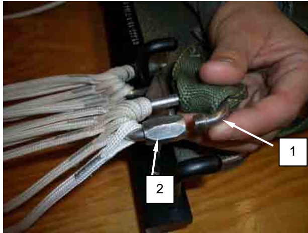
Figure 3. Replacing a Main Canopy Suspension Line.
