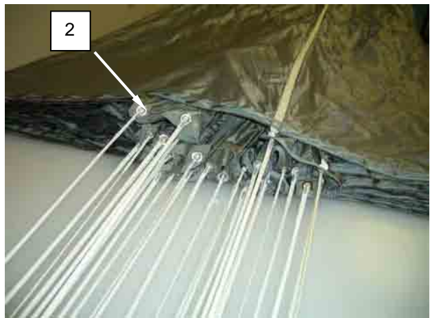
Figure 27. Move Slider and Place Neatly in Air Channel.
