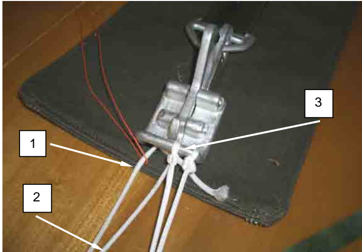
Figure 2. Routing the Ticket 8/4 Cotton Thread through Loop of Apex Hook Lanyard.
