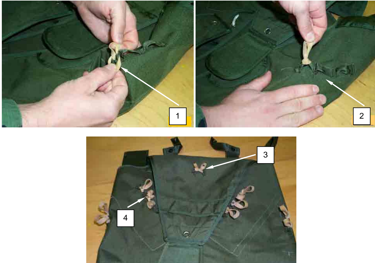
Figure 8. Attaching Retainer Bands to Static Line Stow Bars and Static Line Slack Retainer.
