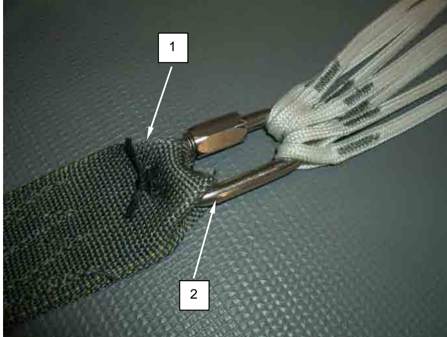
Figure 8. Positioning Riser to Lower Portion of Connector Link.
