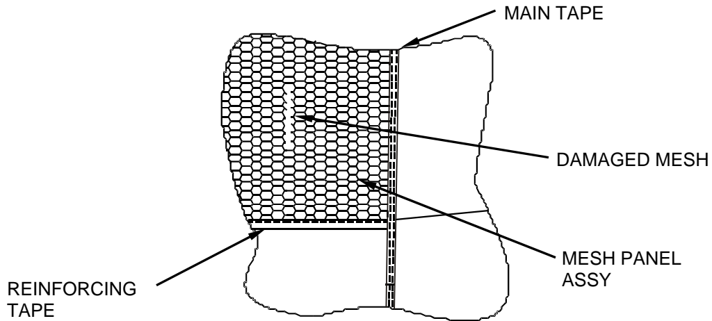
Figure 1. Repair Damaged Mesh Panel.
