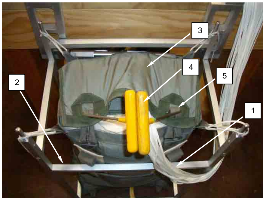
Figure 45. Secure Locking Stow Panel with Stow Hooks.
