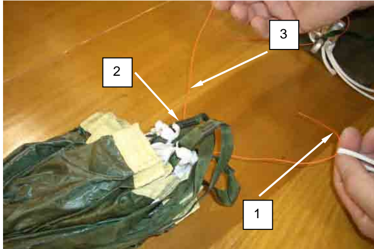
Figure 41. Pulling the Apex Hook Lanyard through the Apex Loops.
