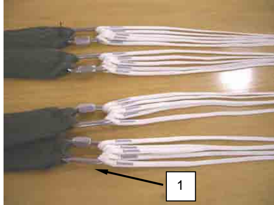
Figure 11. Rotating Risers to Lower Portion of Connector Link.
