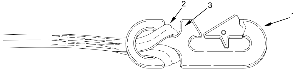
Figure 7. Snap Hook through Static Line Loop Secured with Girth-Hitch.
