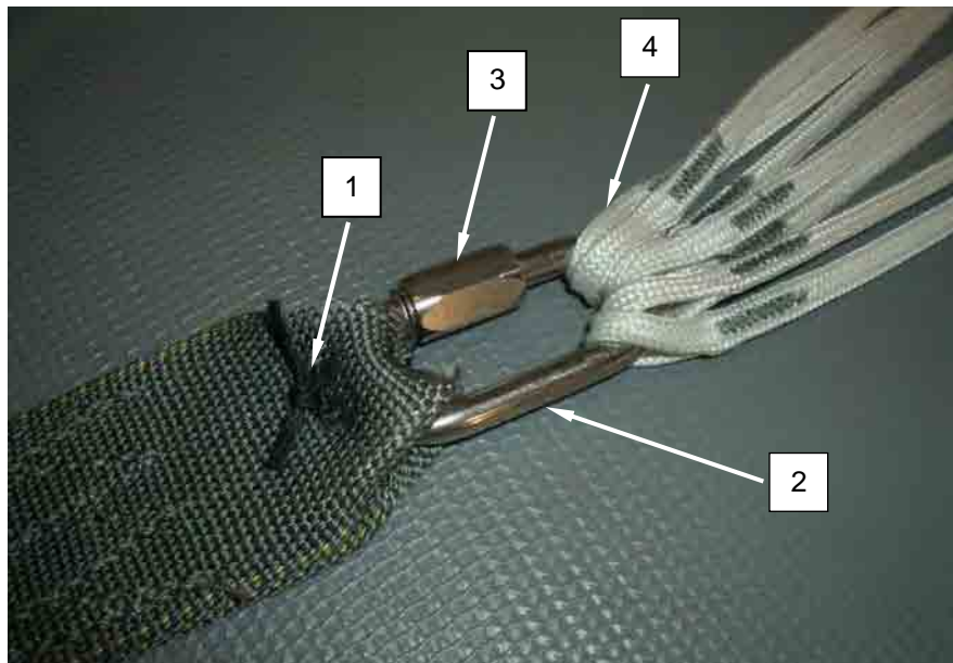
Figure 1. Replacing Main Canopy Suspension Line Connector Link.
