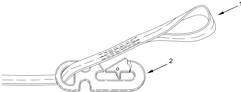
Figure 4. Pass Loop End of Static Line Extension through Opening in Base of Snap Hook.
