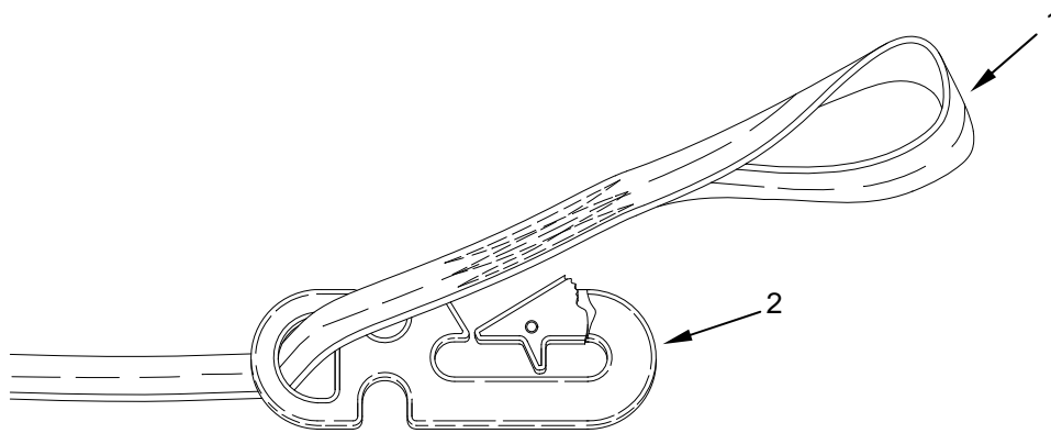
Figure 5. Pass 3½-Inch Loop End of Static Line through Opening in the Base of Snap Hook.
