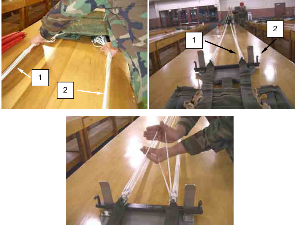
Figure 16. Performing a Four Line Check.
