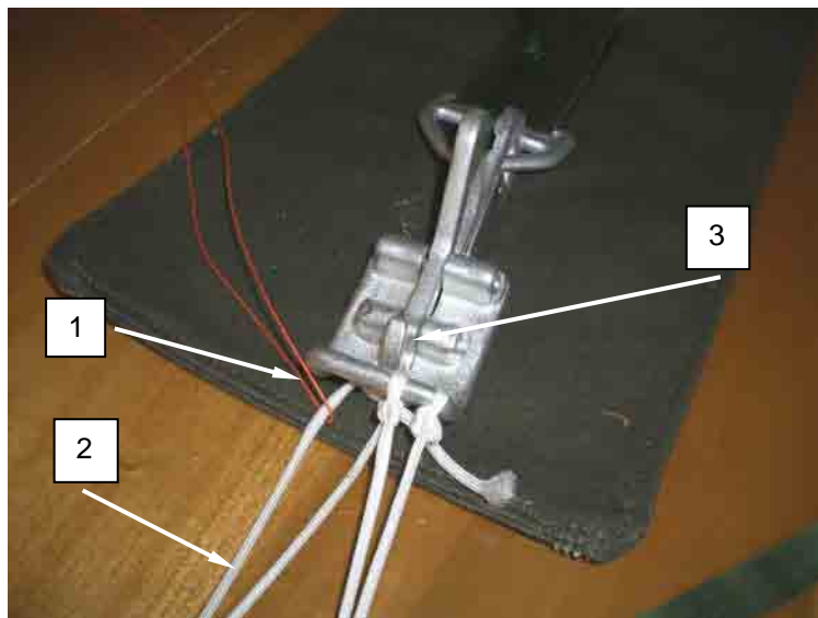
Figure 2. Routing the Ticket 8/4 Cotton Thread through Loop of Apex Hook Lanyard.
