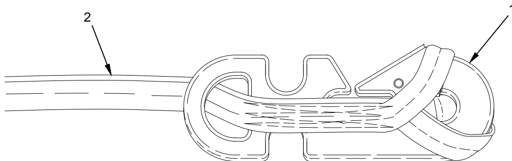
Figure 32. Passing Top of Snap Hook through Loop End of Static Line.
