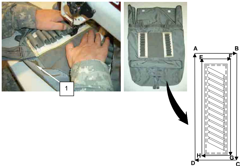
Figure 11. Sew Second Row of Stitching Around Suspension Line Stow Loop Panel.
