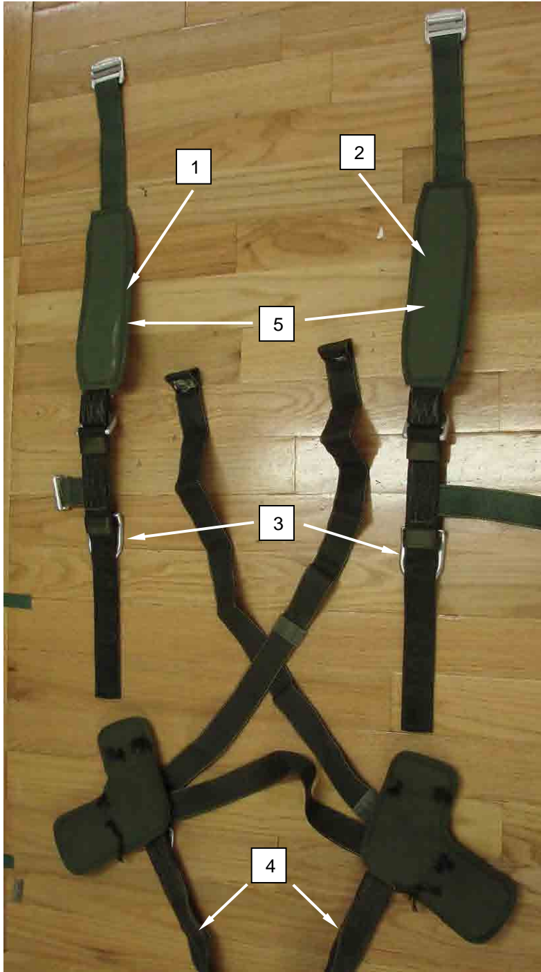
Figure 6. Layout of Harness Assembly Components.
