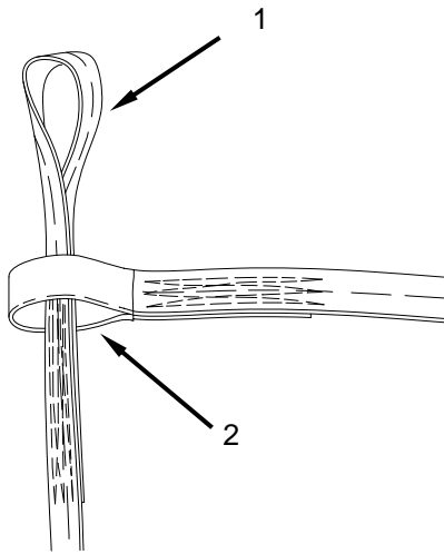
Figure 9. Pass the 3½-Inch Loop on the Static Line through the 2-Inch Buffer Loop.
