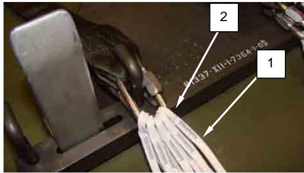
Figure 2. Attaching New Suspension Line to Connector Link.
