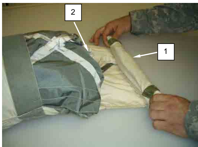
Figure 35. Roll Bridle Line Stowage Panel to Edge of S-Folded Center Section.
