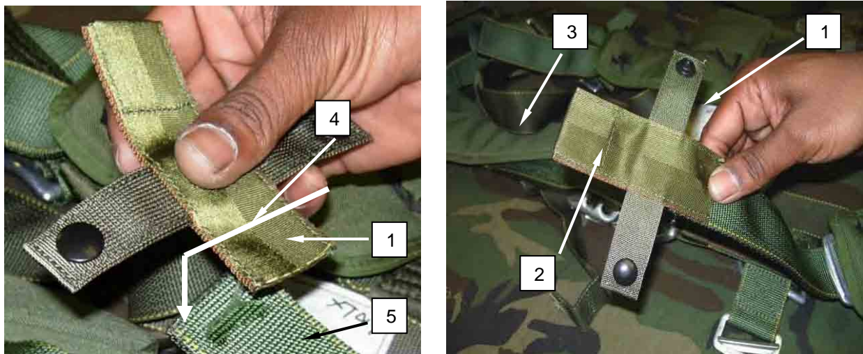
Figure 11. Proper Positioning of the Tuck Tab Assembly.
