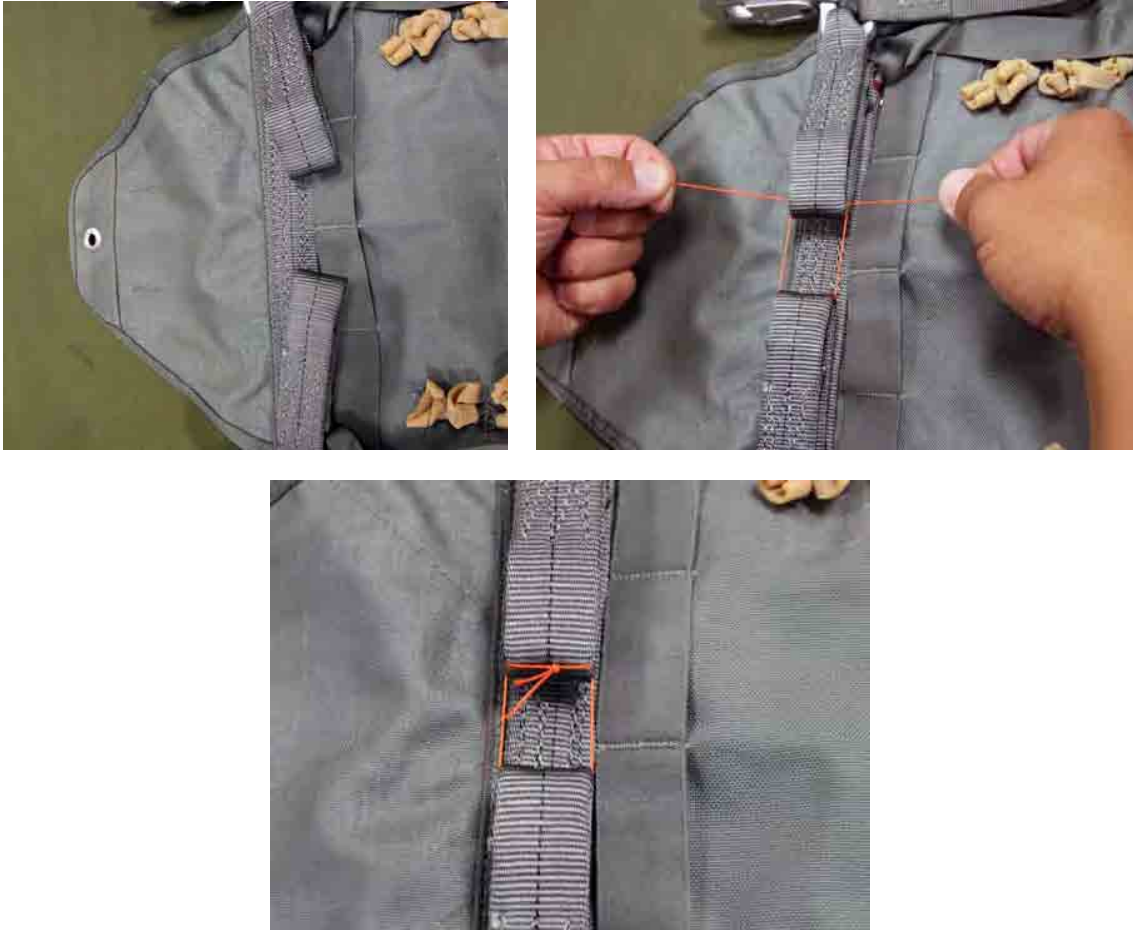
Figure 16. Securing the Excess Spreader Bar Fold-over.
