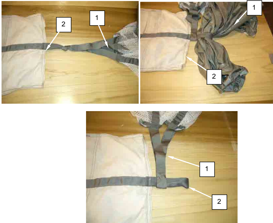
Figure 1. Remove Main Drogue Parachute.
