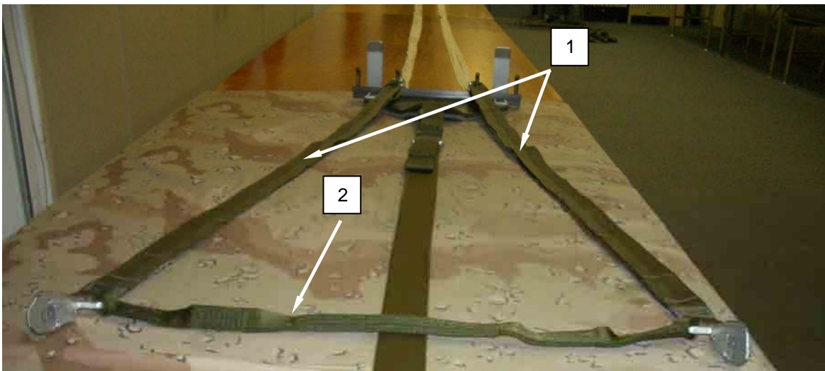
Figure 19. Reserve Risers.
