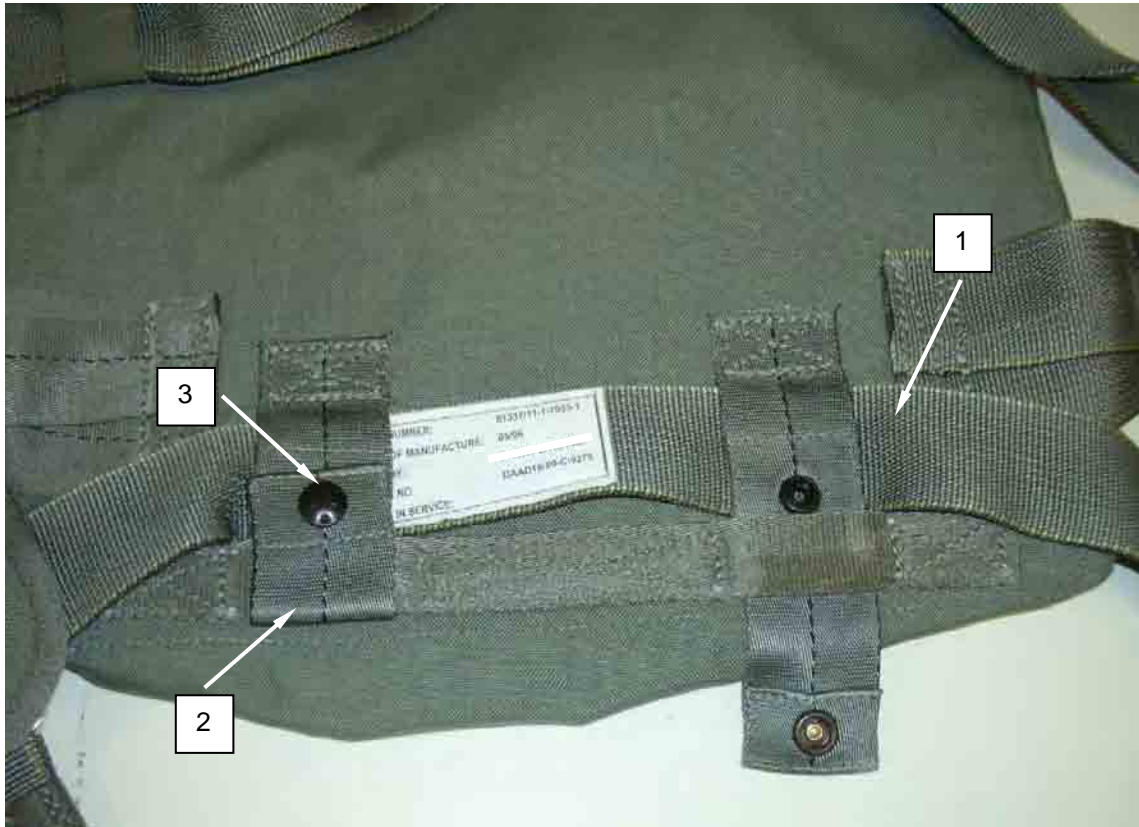
Figure 5. Securing Horizontal Back Strap.
