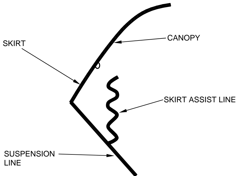
Figure 13. Skirt Assist Lines at High Speed.
