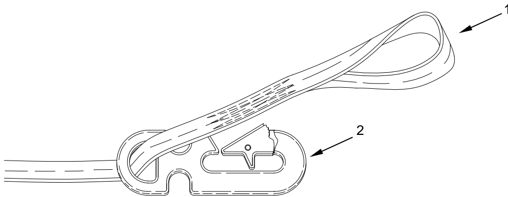
Figure 6. Pass 3½-Inch Loop End of Static Line through Opening in Base of Snap Hook.
