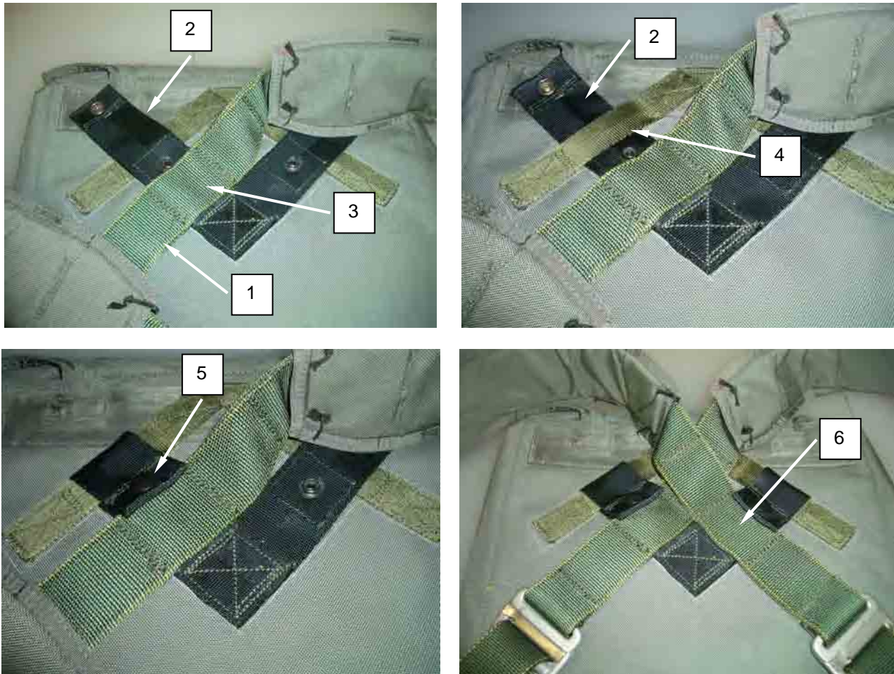
Figure 15. Securing Diagonal Backstraps.
