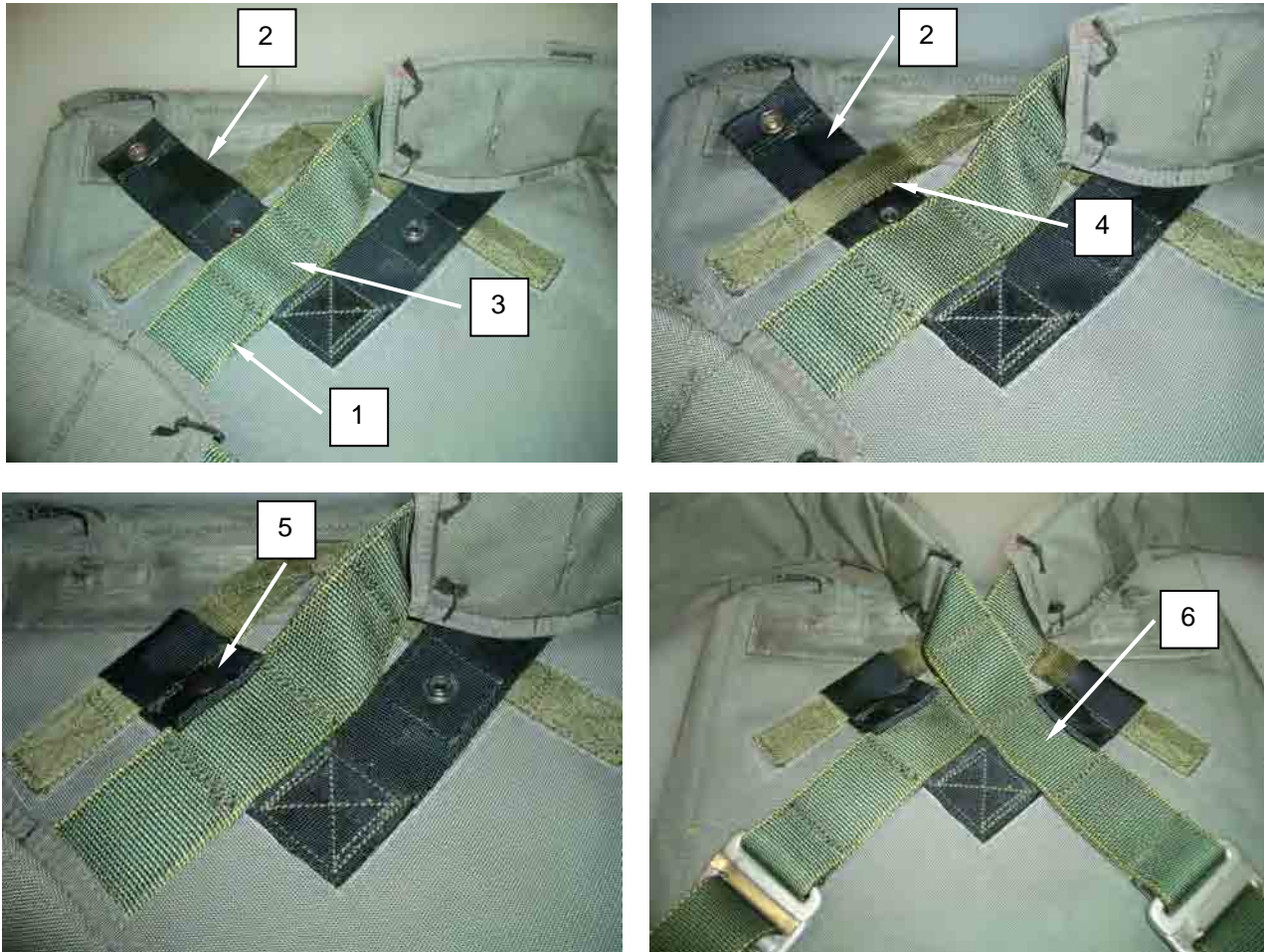
Figure 7. Route Tuck Tabs, Close Snap Fastener, and Snap Fastener Secured.
