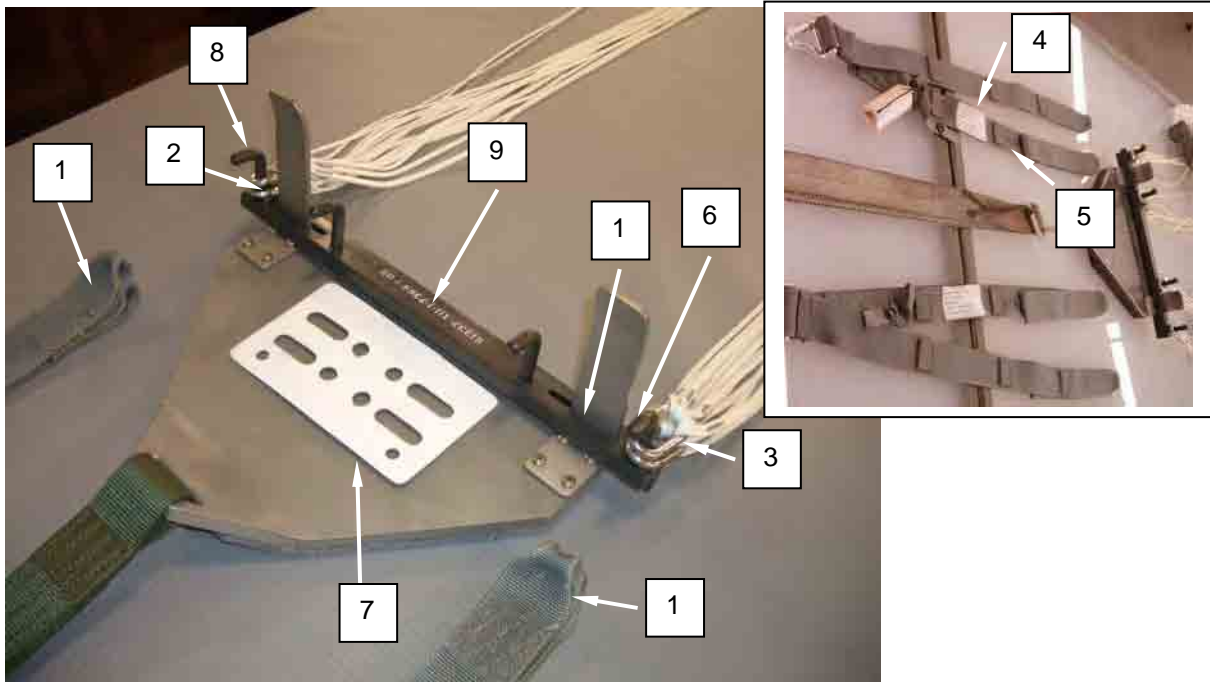
Figure 1. Place Connector Links and Riser Assembly.
