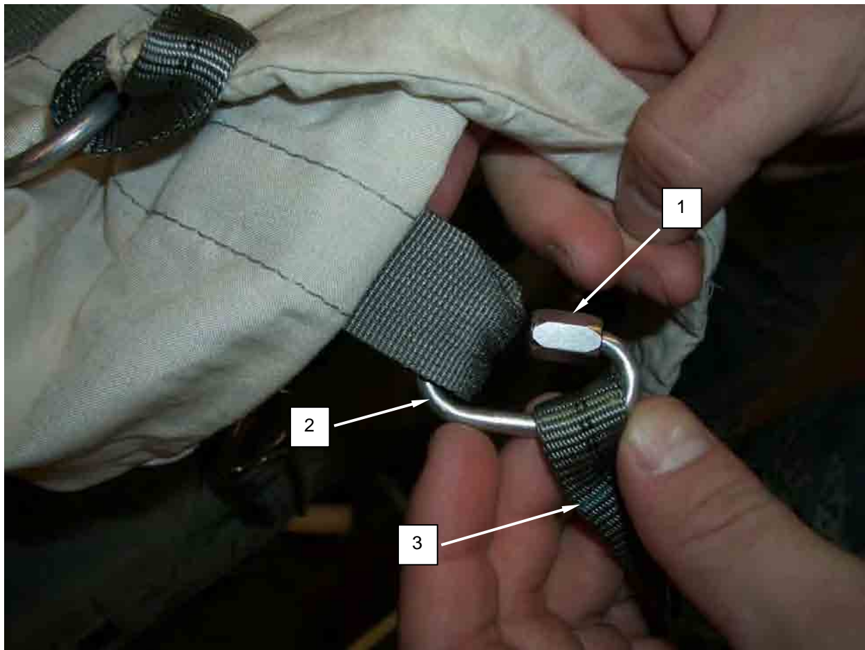
Figure 1. Replacing Connector Links.
