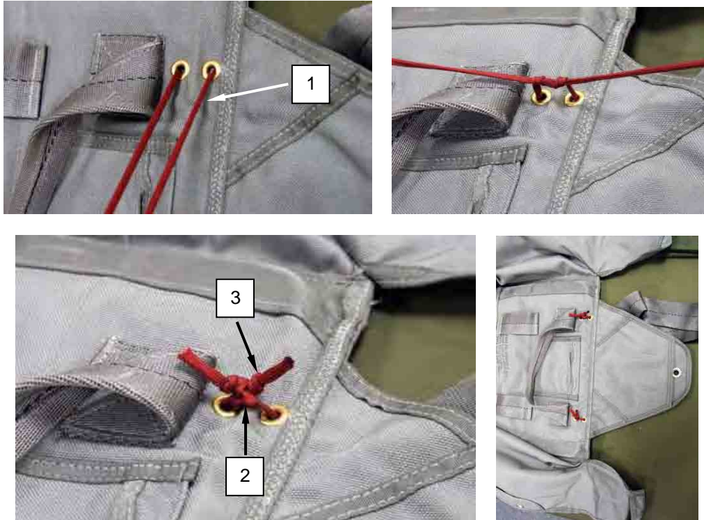
Figure 13. Securing the Spreader Bar on Back Side of Pack Tray.
