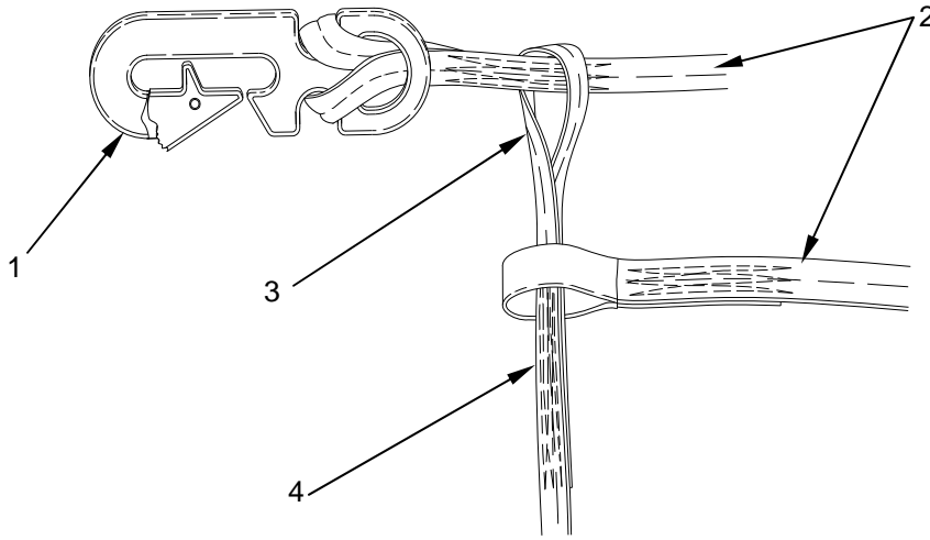
Figure 35. Passing Snap Hook of USL Extension through Loop on Static Line.
