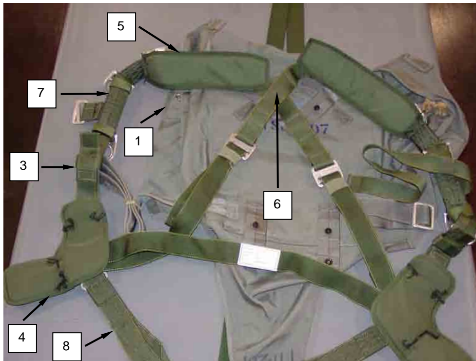
Figure 13. Pack Tray and Harness Assembly.
