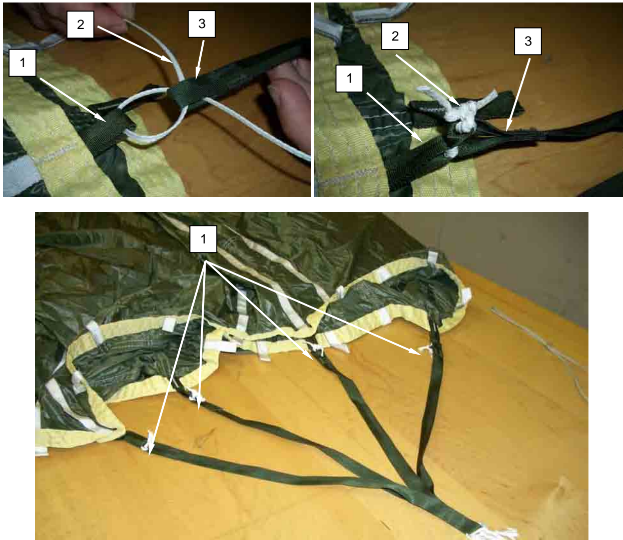
Figure 3. Attaching Extractor Bridle Lines.
