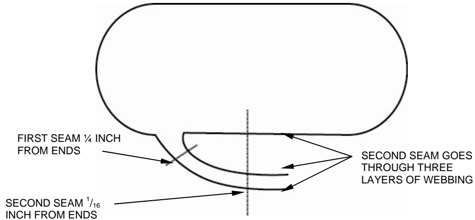
Figure 3. Loop Stitching Locations.
