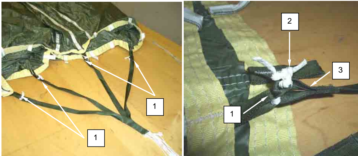
Figure 1. Remove Cord from Apex Extractor Attaching Loop.
