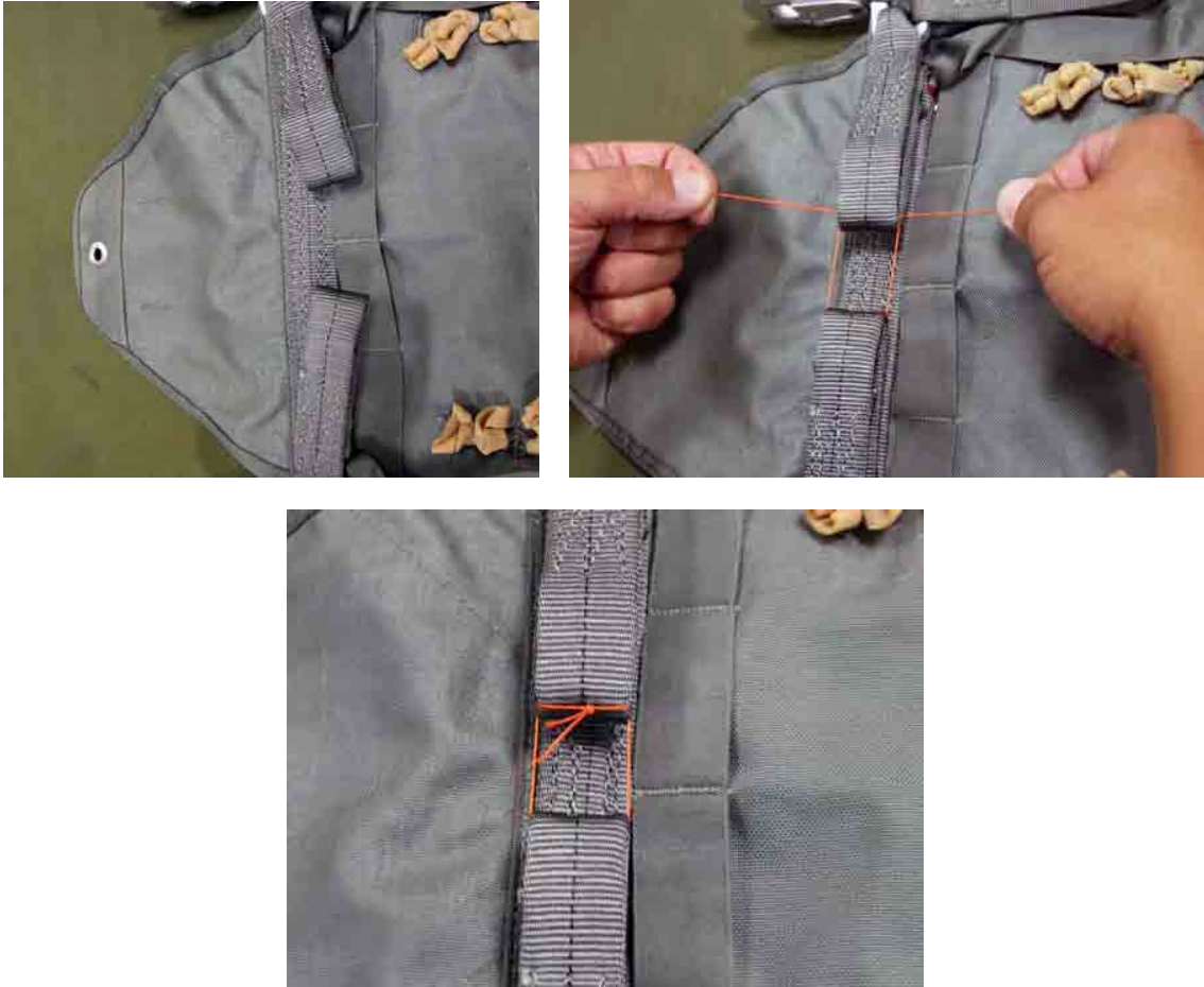
Figure 14. Securing the Excess Spreader bar Fold-over.
