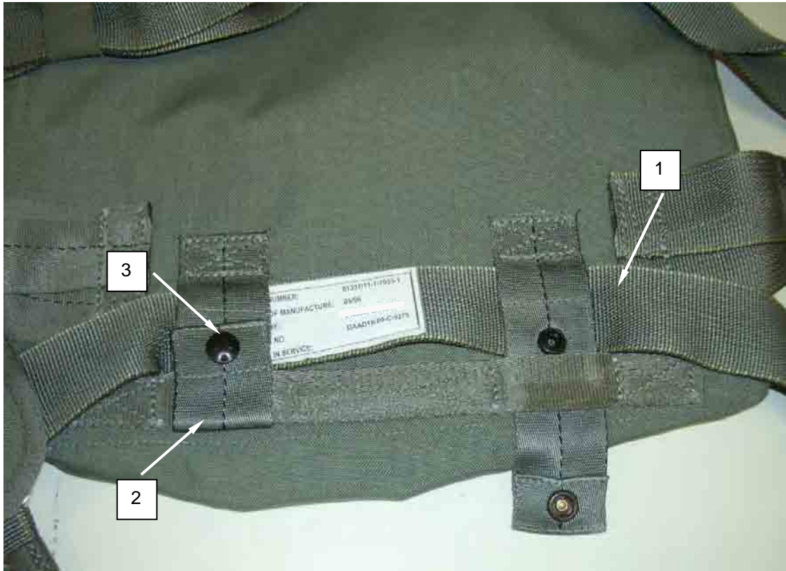
Figure 6. Securing Horizontal Back Strap.
