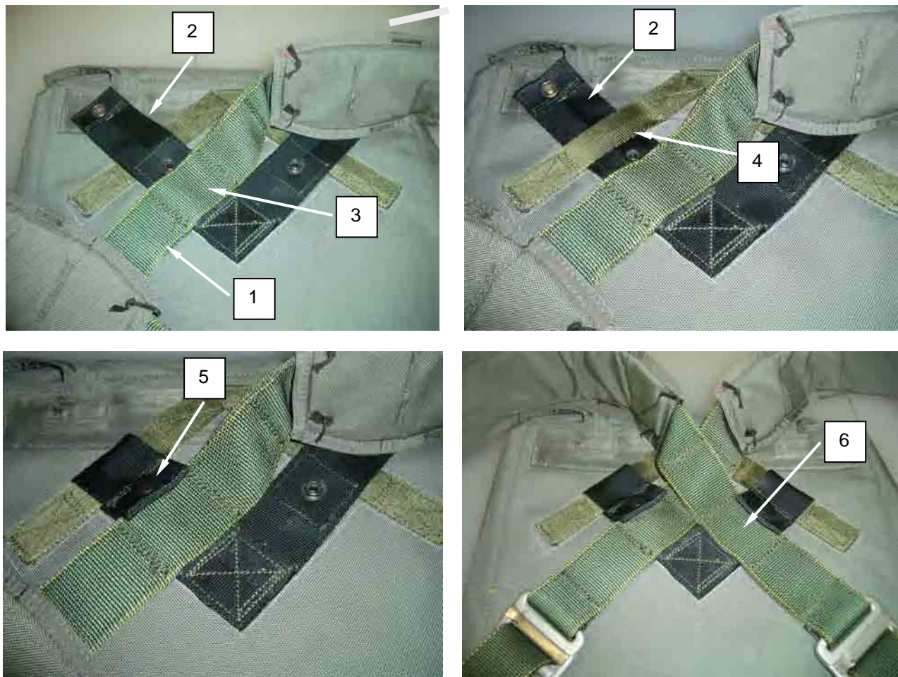
Figure 17. Securing Diagonal Back Straps.
