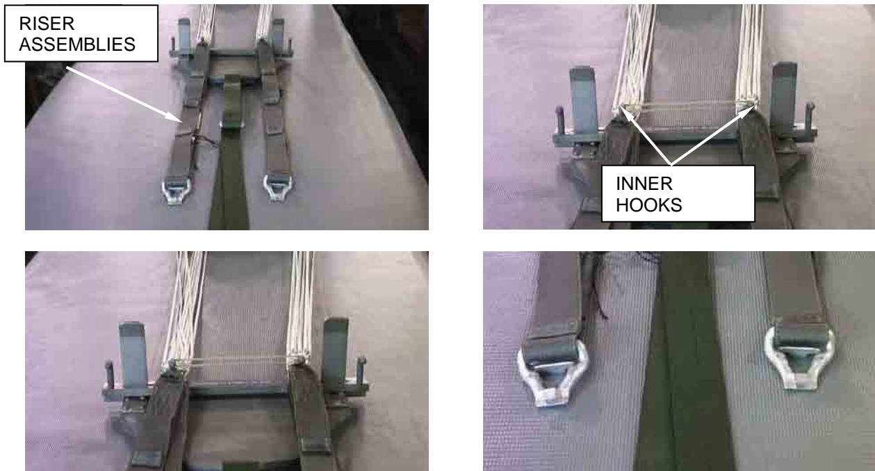
Figure 4. Attach the Riser Assemblies.
