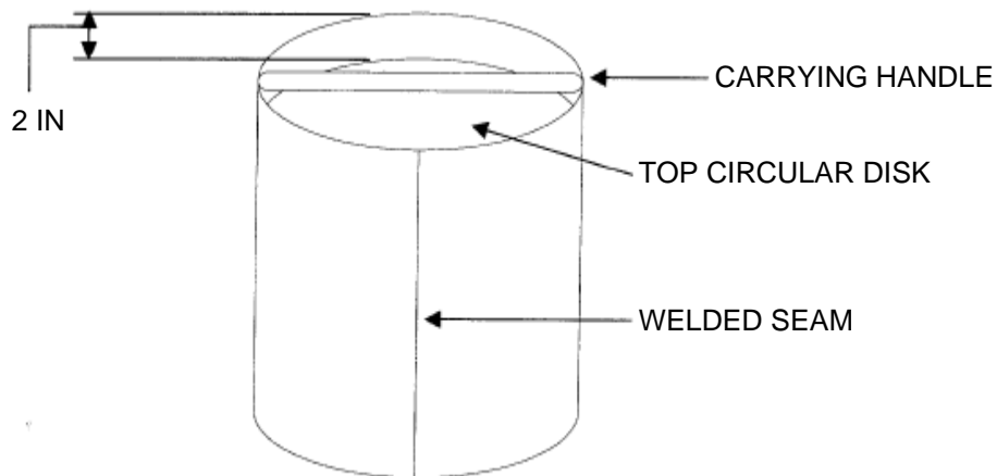
Figure 4. Fabricating 32-Pound Weight.
