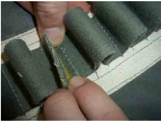
Figure 4. Prepare Stow Loop Panel for Sewing.
