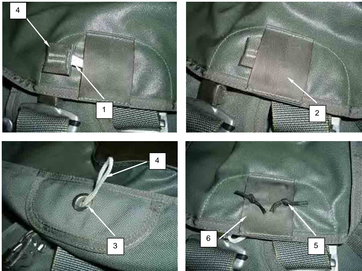
Figure 17. Routing Main Closing Loop under Protective Cover, through Grommet, and Tacking Both Sides.
