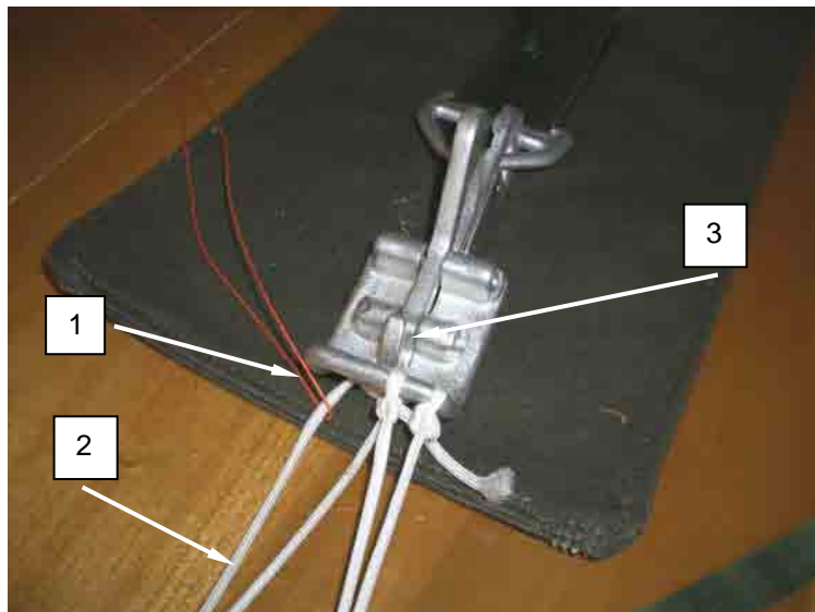
Figure 5. Routing the Ticket 8/4 Cotton Thread through Loop of Apex Hook Lanyard.
