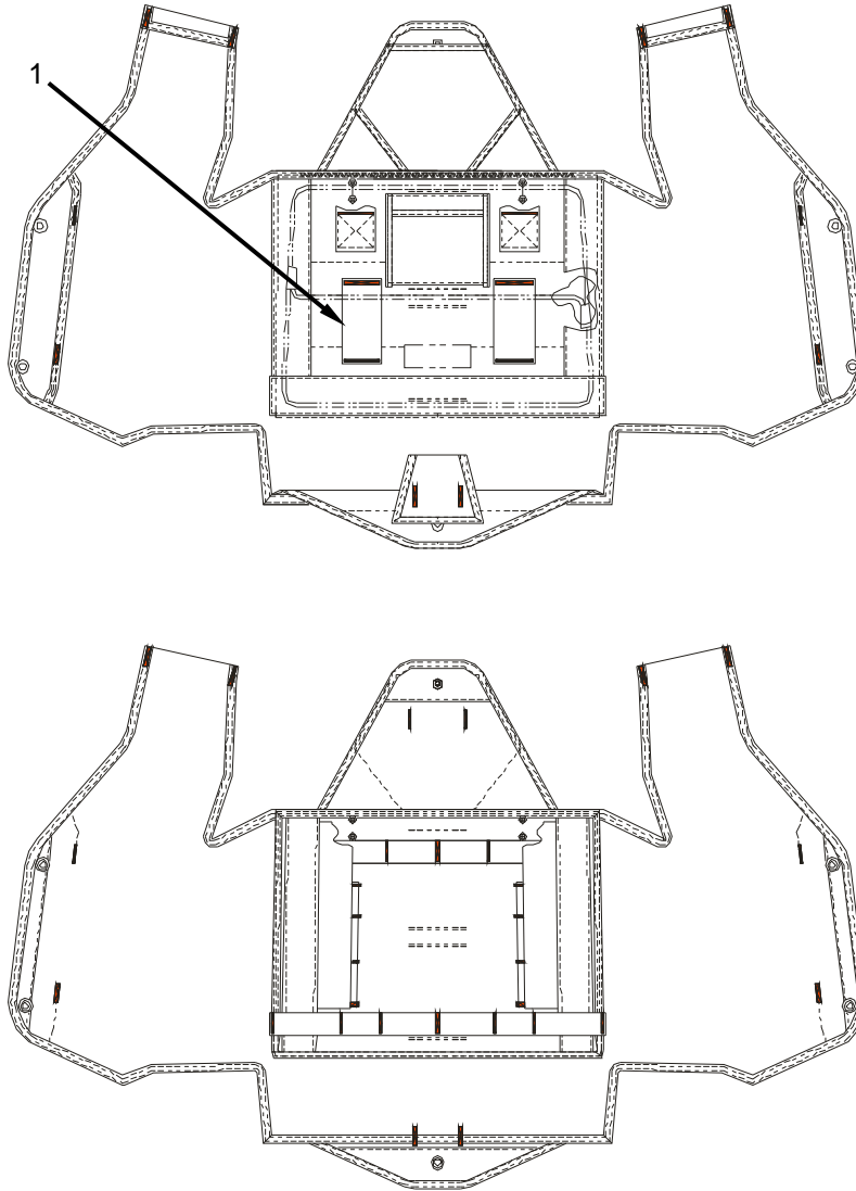
Figure 1. Reserve Pack Tray Waistband Retainers.
