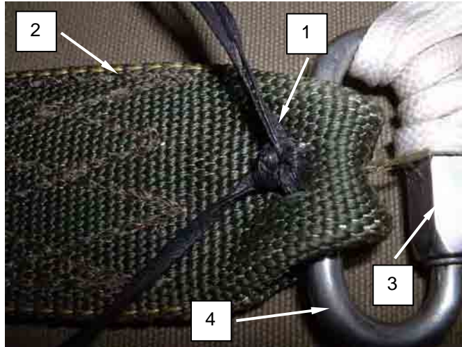
Figure 4. Remove Tacking.
