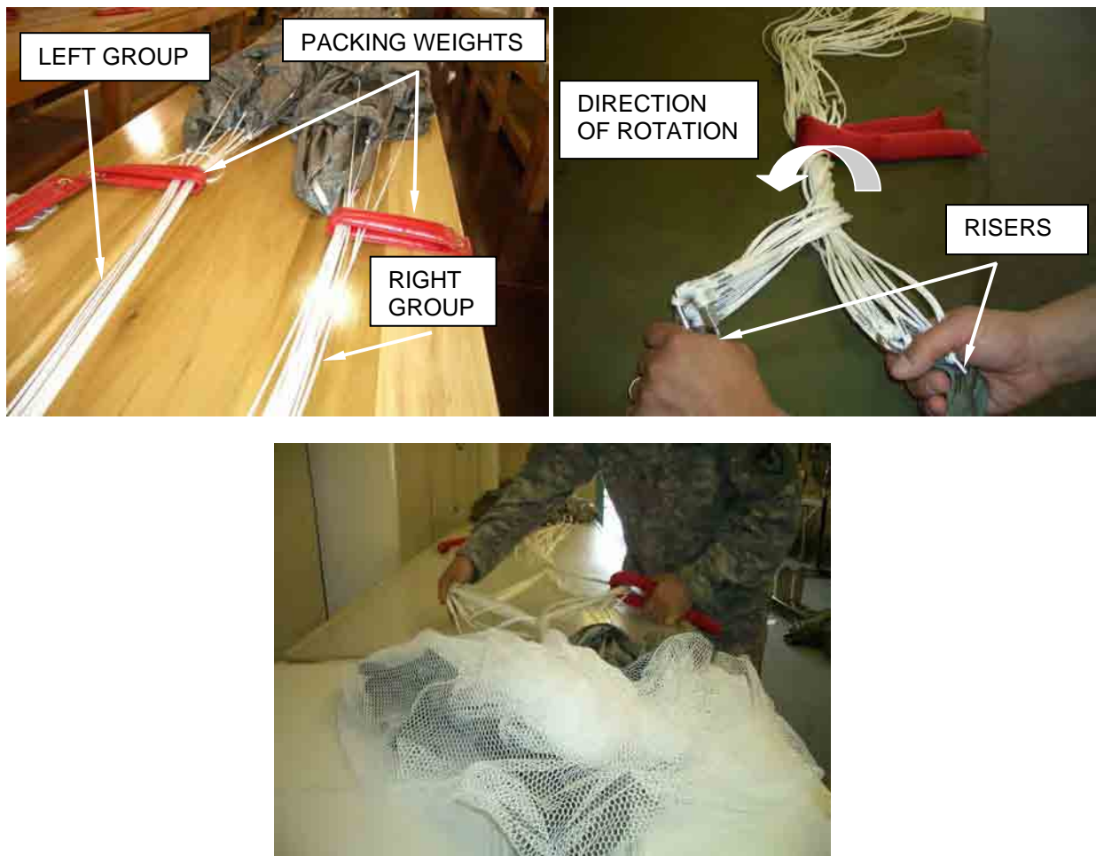
Figure 5. Removing Turns, Tangles, or Twists from Suspension Lines.
