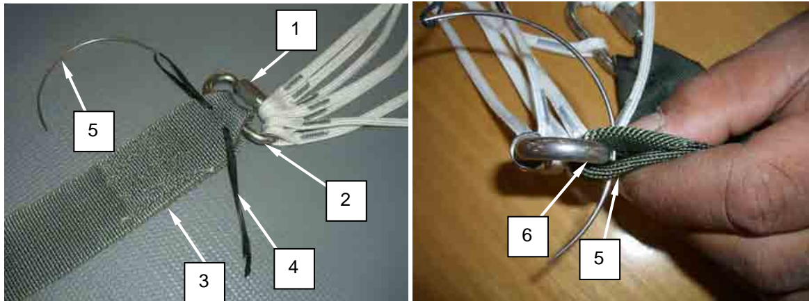
Figure 6. Tightening Connector Link Barrel Nut and Tacking Each Riser.
