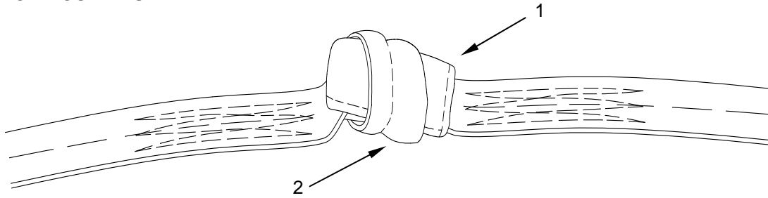
Figure 11. Secure 5-foot Extension to Static Line with Taut Girth-Hitch.
