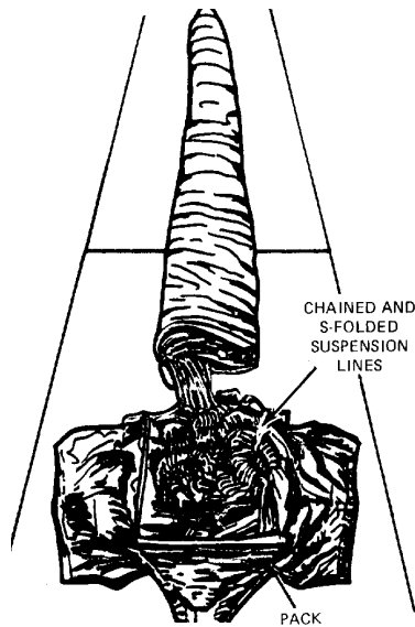
Figure 2. Suspension Lines Stowed on Pack.
