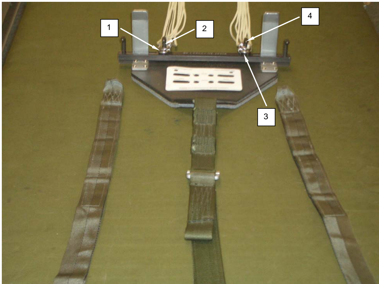
Figure 7. Riser Connector Links.
