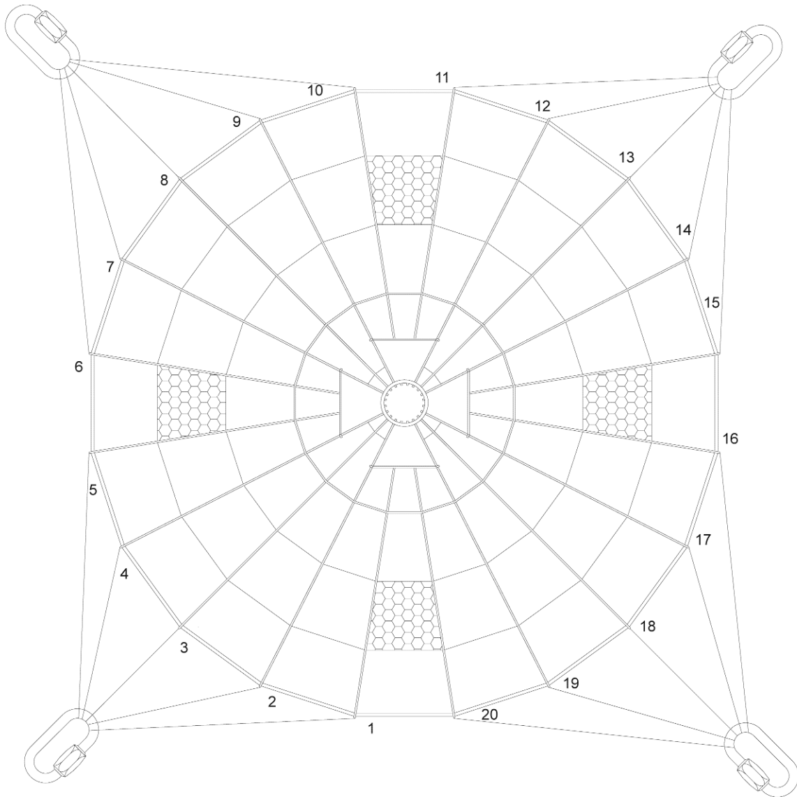
Figure 27. T-11 Reserve Canopy.
