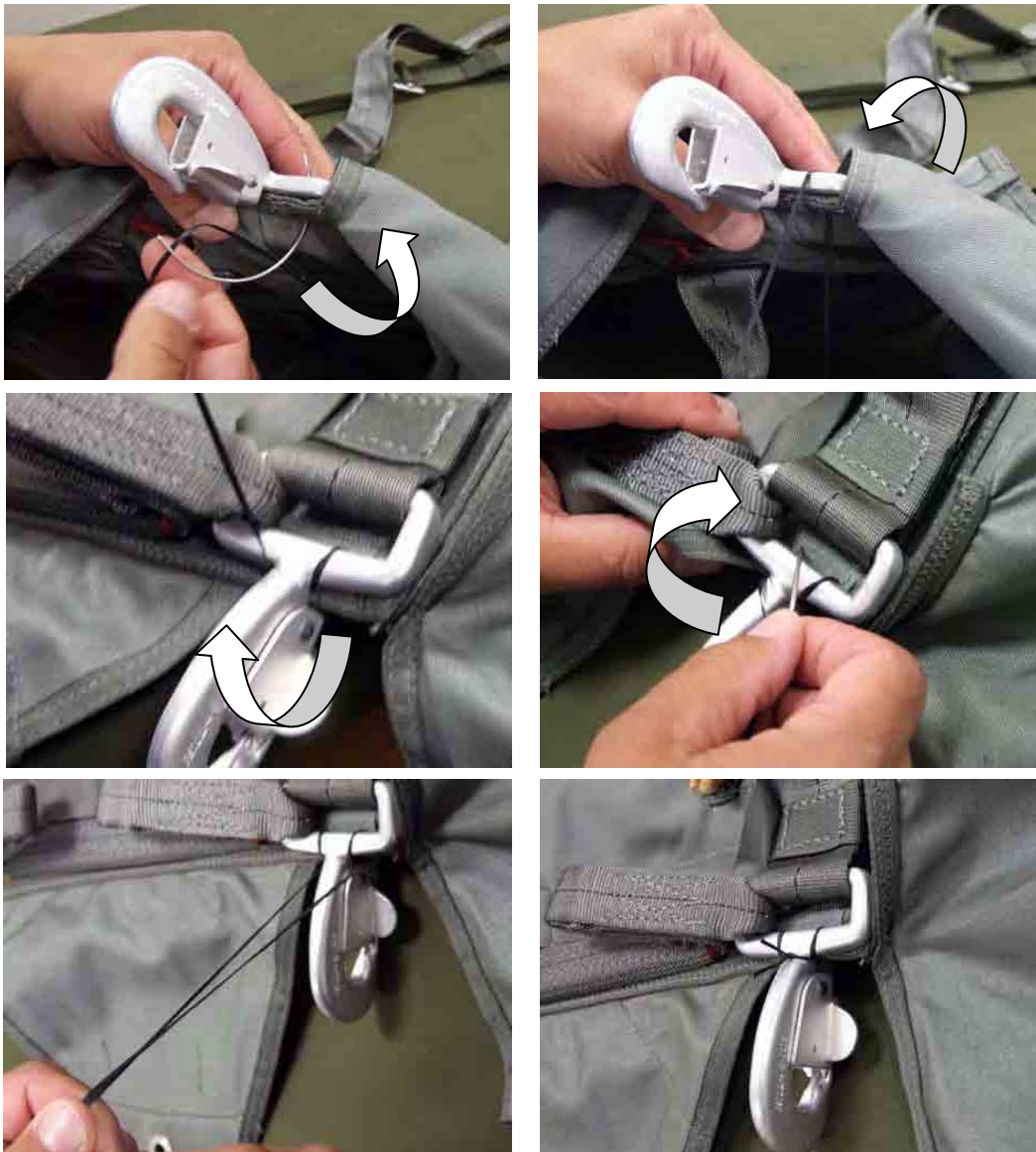
Figure 15. Securing Connector Snaps To Pack Tray.
