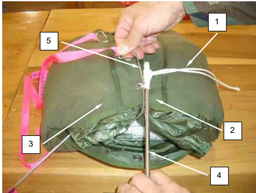
Figure 54. Exposing Closing Loops and Inserting Temporary Pin.
