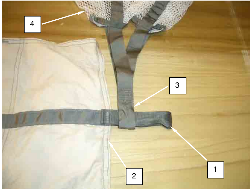
Figure 19. Sliding Looped End of Drogue Parachute over Drogue Parachute Attaching Loop.
