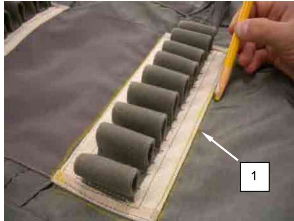
Figure 6. Mark Damaged Suspension Line Stow Loop Panel on Deployment Bag.
