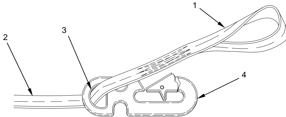
Figure 31. Passing Loop End of Static Line through Base of Snap Hook.
