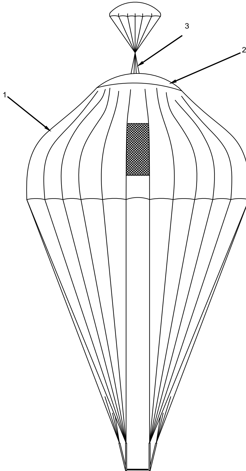
Figure 11. T-11 Reserve Parachute Assembly.
