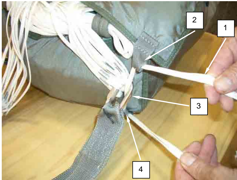
Figure 51. Secure Connector Links with Cotton Webbing.
