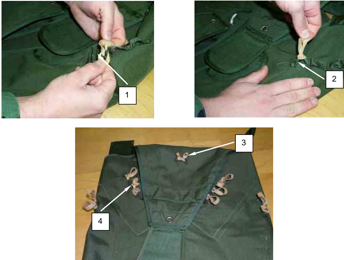
Figure 16. Attaching Retainer Bands to Static Line Stow Bars and Static Line Slack Retainer.
