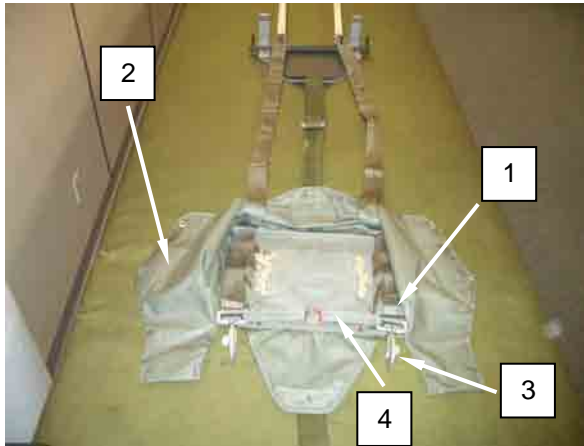
Figure 1. Remove Reserve Pack Tray from Reserve Canopy Risers.
