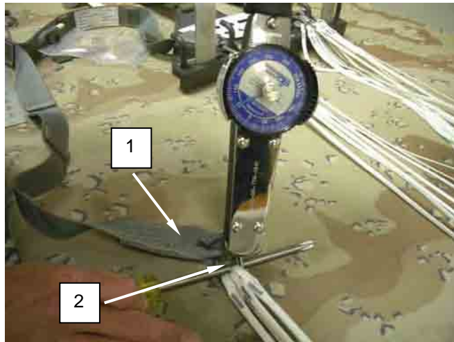
Figure 7. Tighten Barrel Nut on Connector Link.
