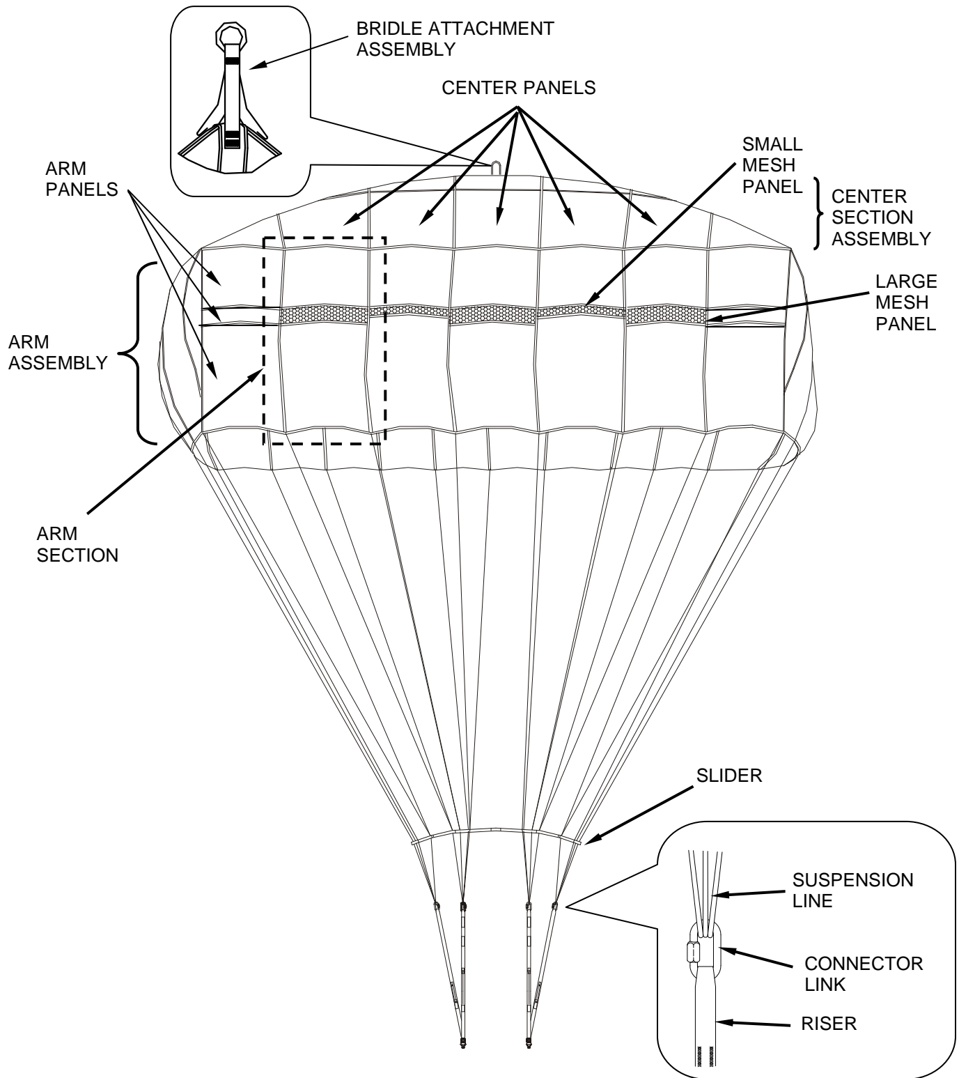
Figure 1. Main Canopy.
