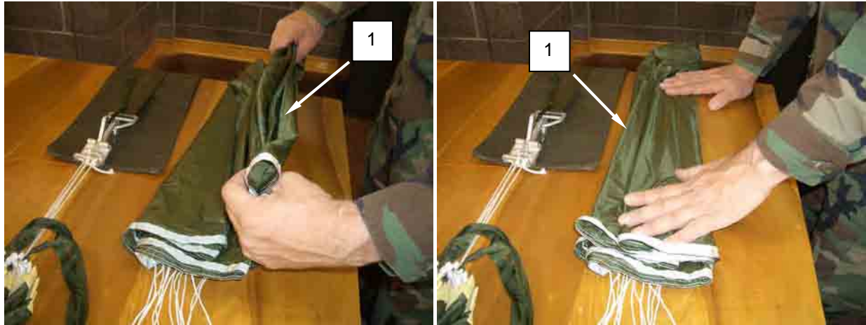
Figure 30. Folding the Extractor Canopy into Thirds.
