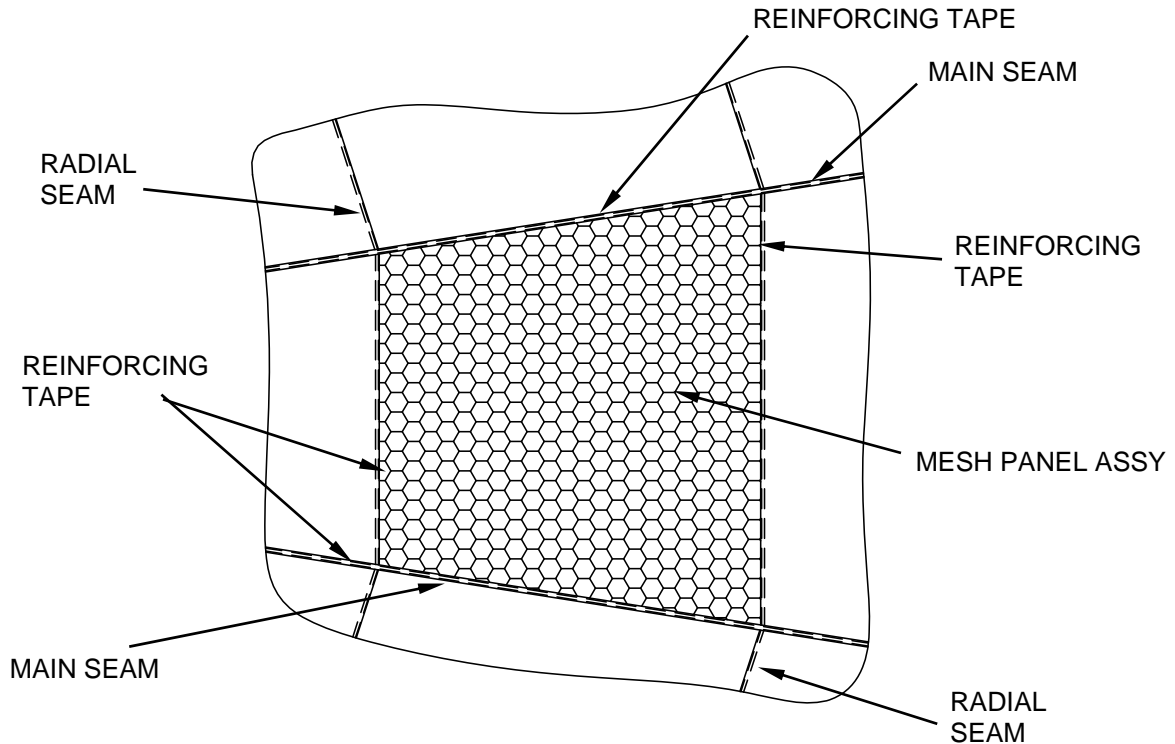
Figure 4. Replace Damaged Mesh Panel.
