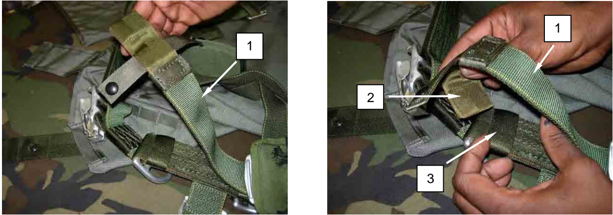
Figure 14. Upper Main Lift Web Assemblies Placed on Small Size Setting.
