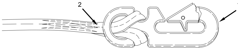
Figure 8. Form a Taut Girth Hitch.
