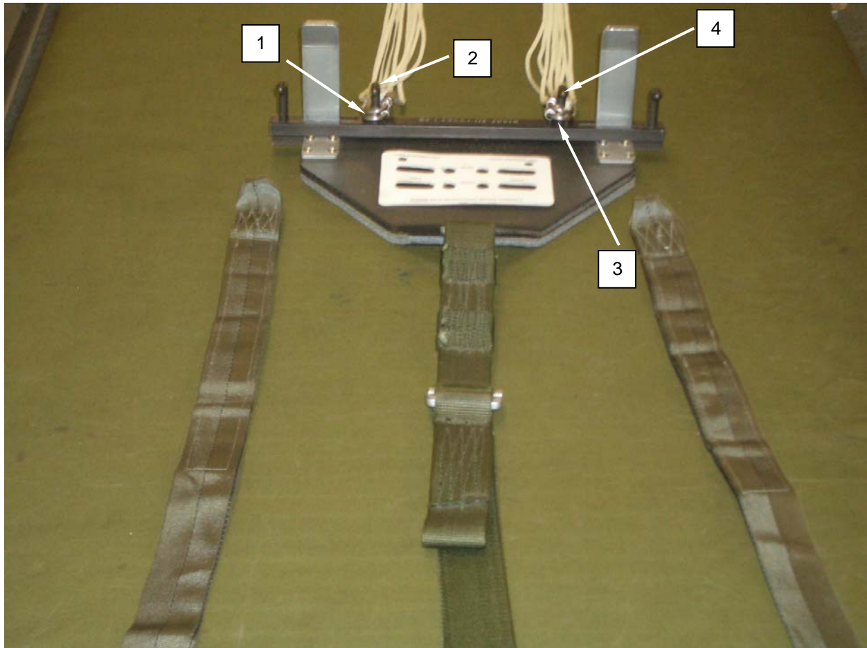
Figure 6. Riser Connector Links.
