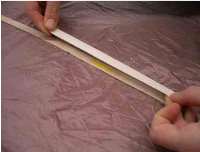
Figure 2. Place the New Material Centered over the Damaged Area.
