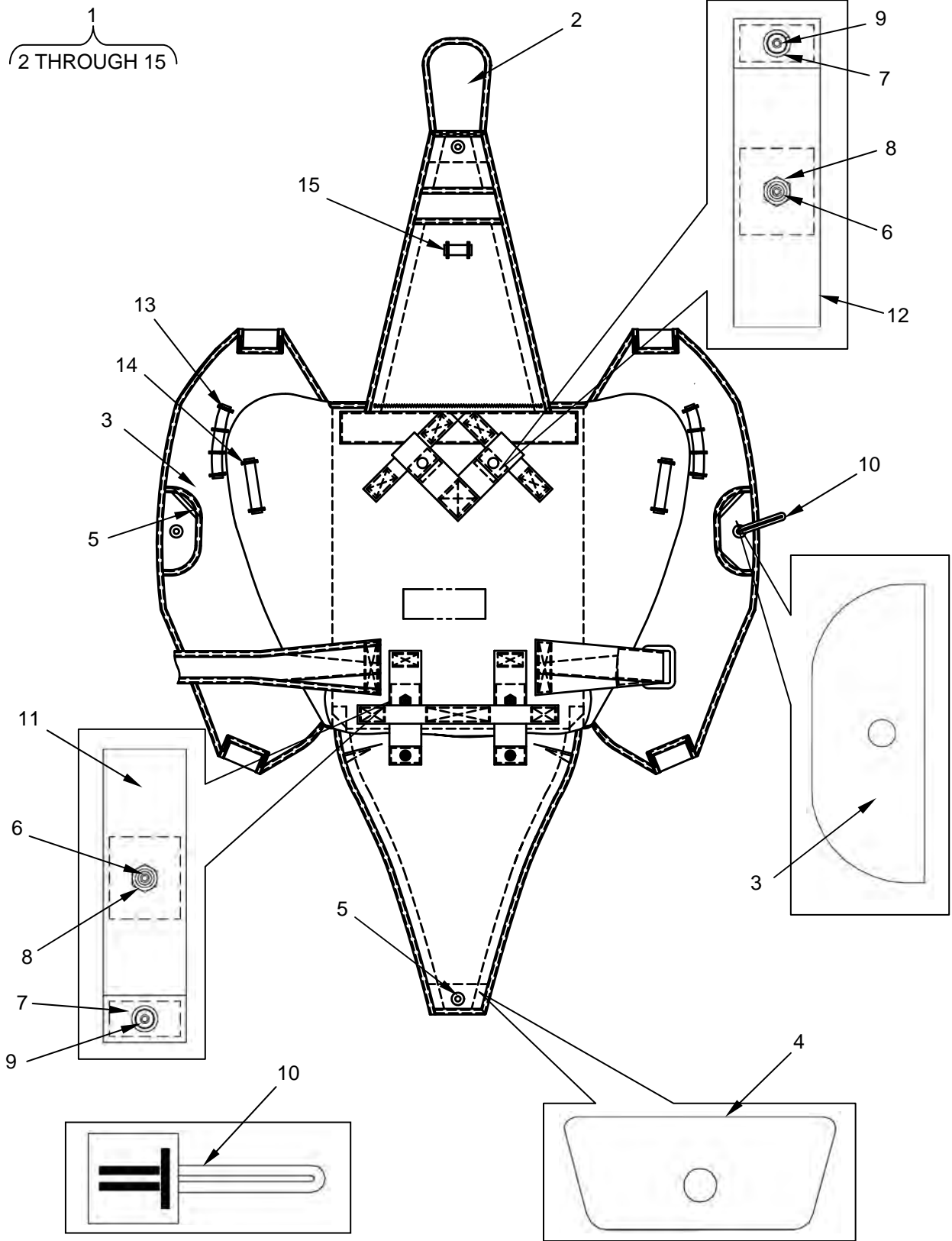
Figure 4. Main Pack Tray.
