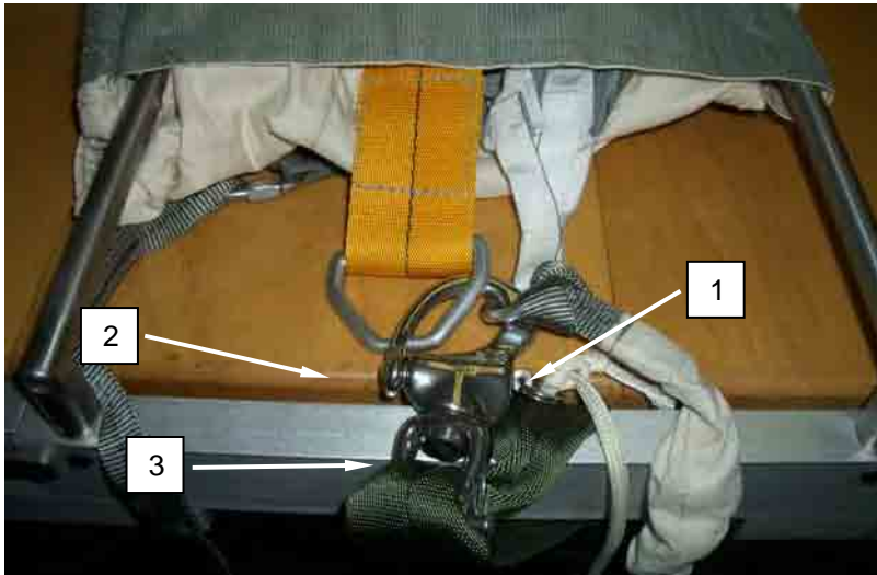
Figure 13. Attach Bridle Ring and Packing Loop Tension Device to Quick Release Hook.
