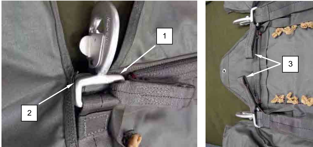
Figure 14. Aligning Top Bar of Snap Hook with Binding Tape and S-Folding Excess Spreader Bar.
