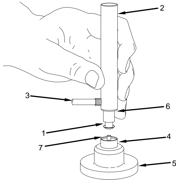
Figure 1. Hand-held Method.
