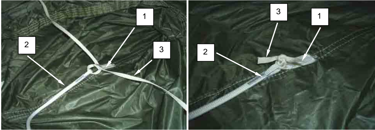
Figure 21. Attaching Skirt Assist Lines.
