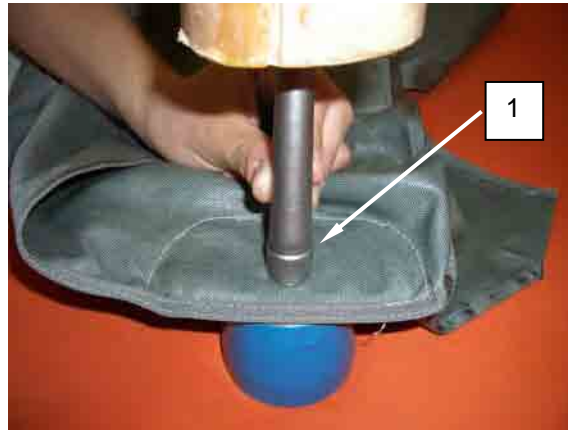
Figure 6. Spread Grommet Barrel.
