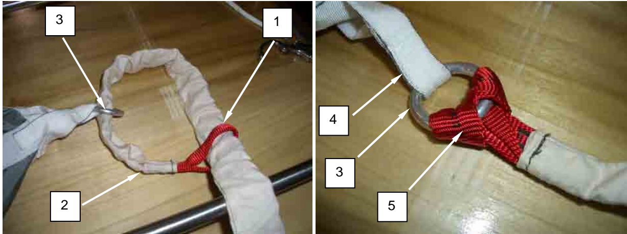
Figure 23. Attaching Bridle Line to Bridle Ring at Top of Canopy.
