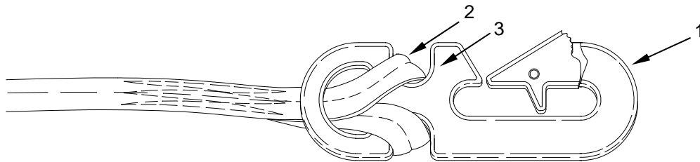
Figure 8. Snap Hook through the Static Line Loop Secured with Girth-Hitch.
