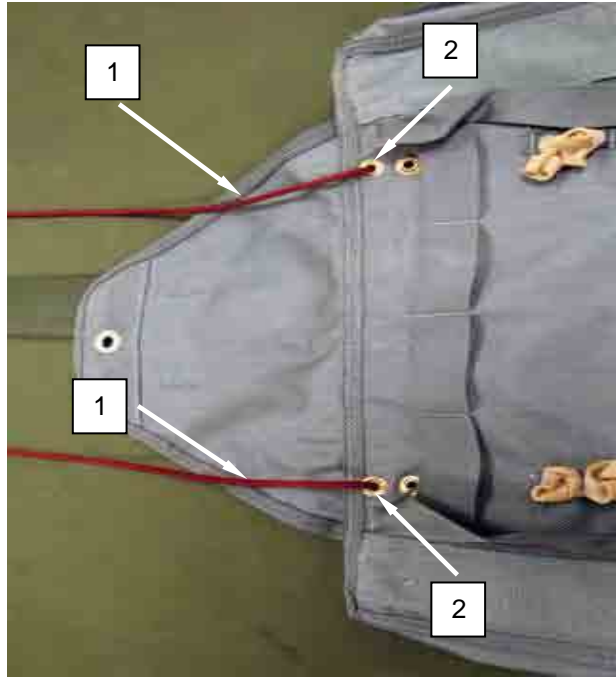
Figure 10. Routing Cord through Top Grommets of Pack Tray.
