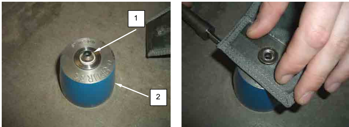
Figure 5. Position Grommet on Die with Barrel Facing up and Place Washer over Grommet Barrel.
