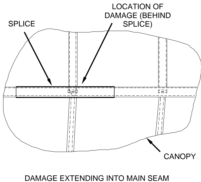
Figure 16. Canopy Repair.
