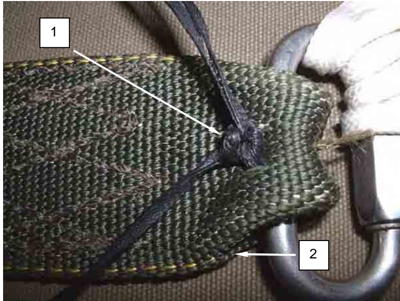
Figure 4. Remove Tacking.
