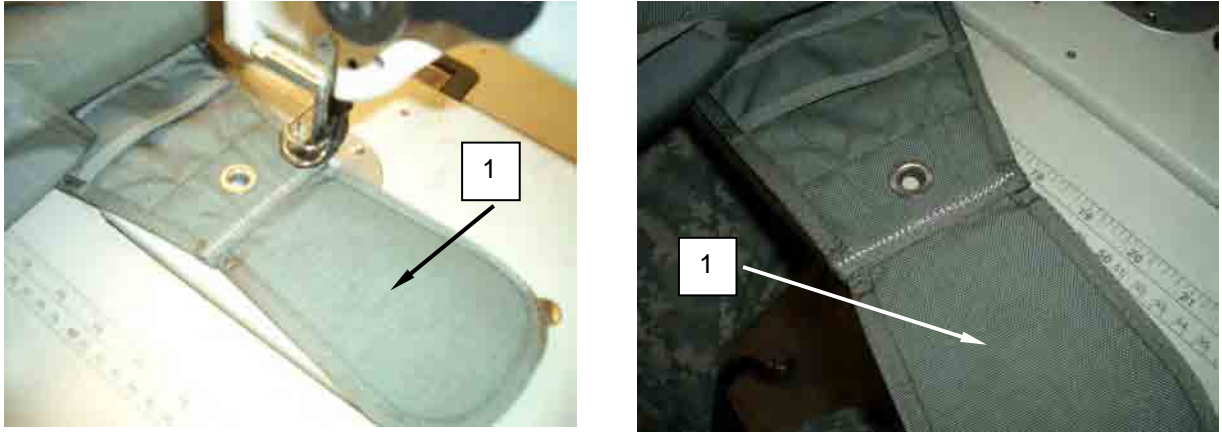
Figure 6. Sew Pin Protector Cover to Binding Tape.
