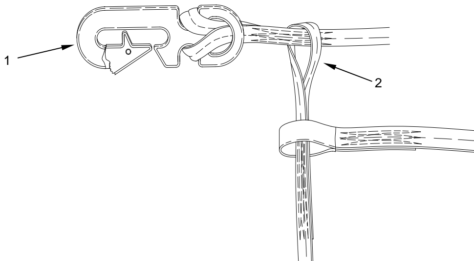
Figure 10. Pass Snap Hook of USL 5-foot Extension through the 3½-Inch Loop on the Static Line.
