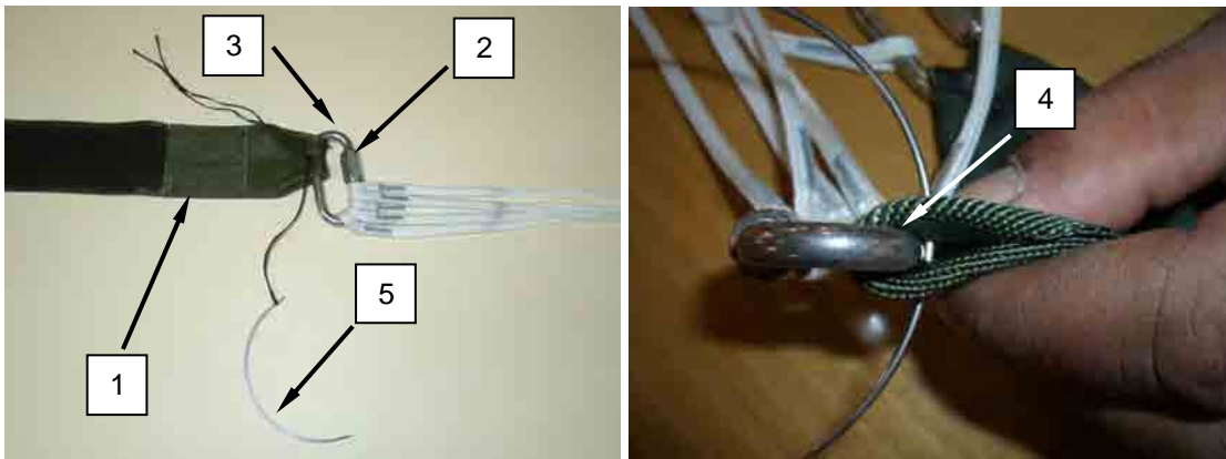
Figure 8. Tacking Reserve Risers.
