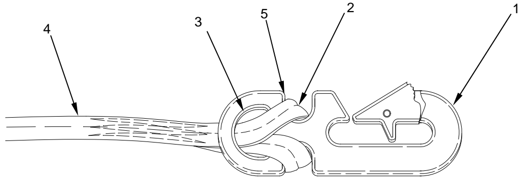
Figure 33. Sliding Loop Down to Bottom of Snap Hook.
