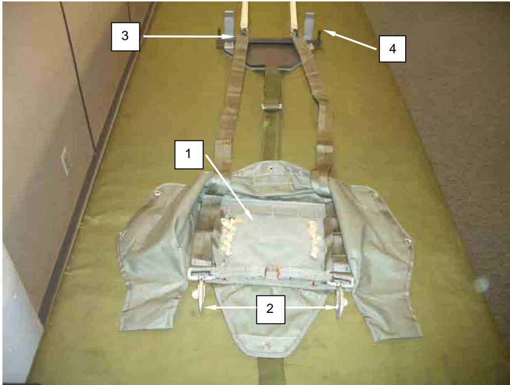
Figure 3. Placing Connector Links on Tension Plate Adapter.
