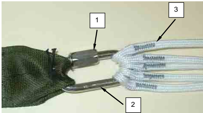
Figure 5. Replace Connector Links.
