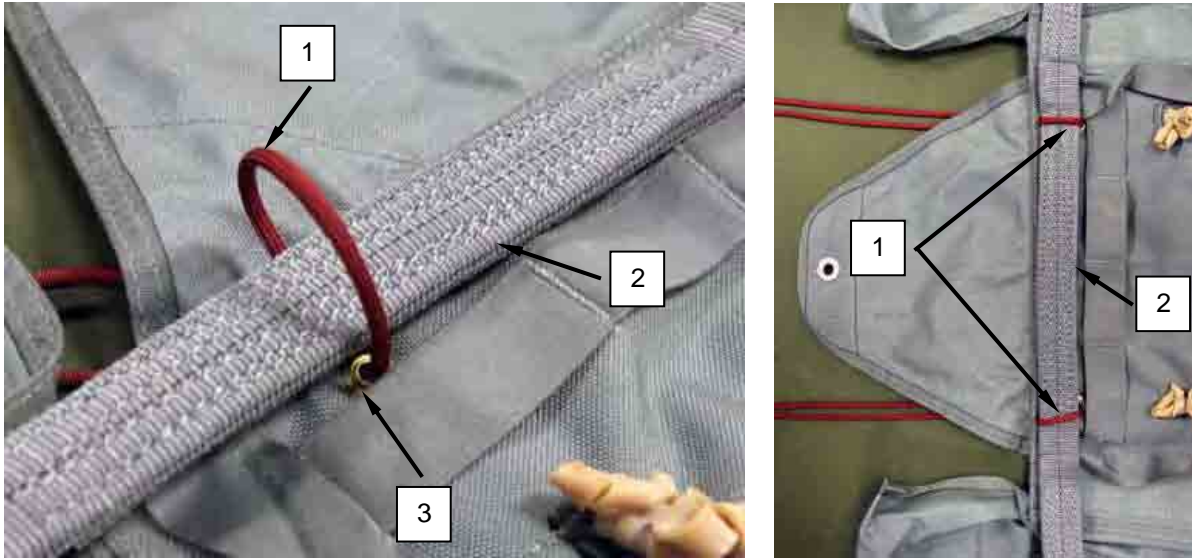
Figure 12. Routing Type III Nylon Cord Over Spreader Bar.
