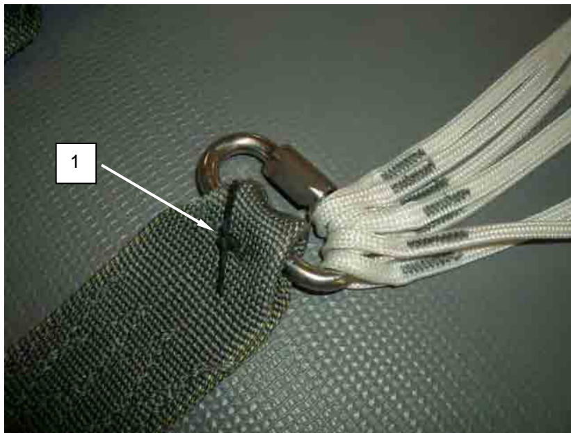
Figure 7. Securing Lacing and Tying Tape with Surgeon's Knot Locking Knot.
