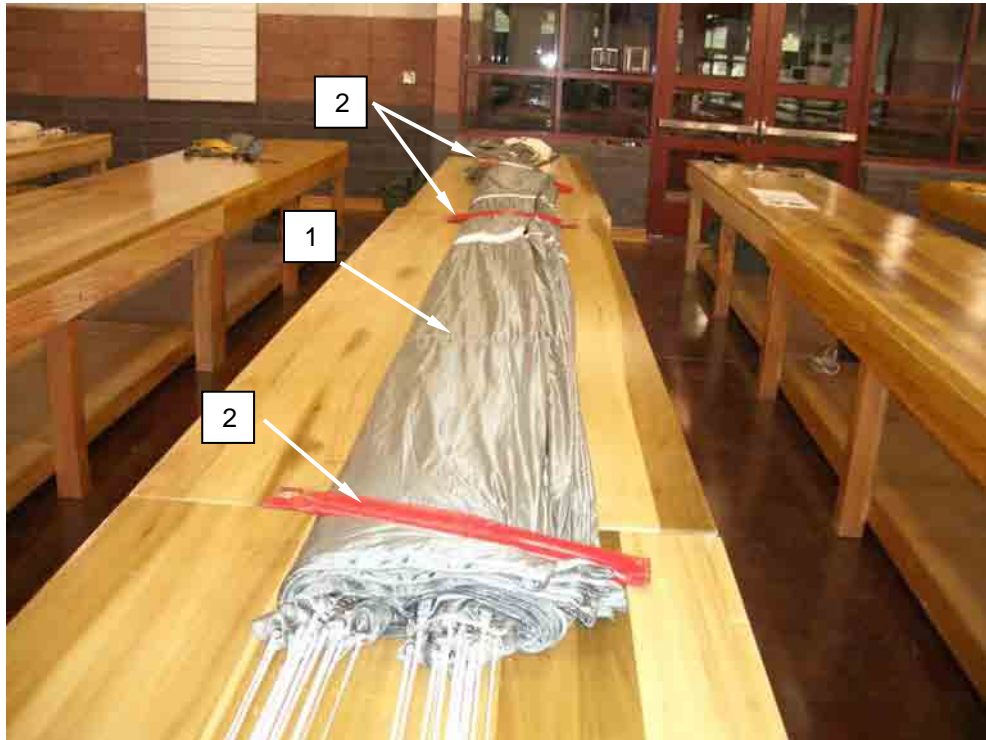
Figure 29. Canopy in Long Fold.
