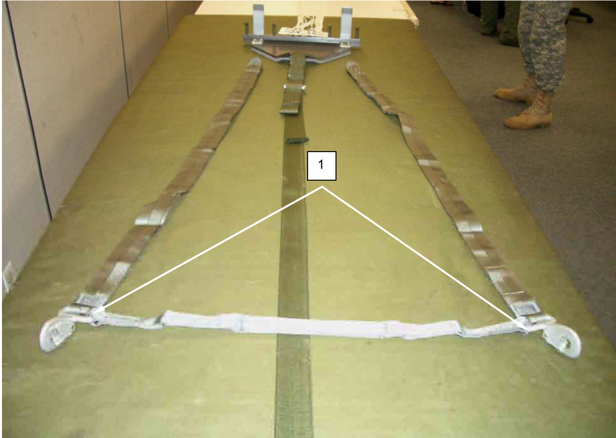
Figure 5. Laying Out Risers.
