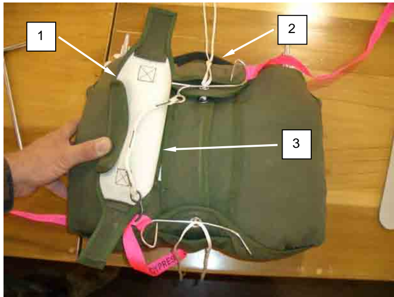
Figure 58. Inserting Right Tuck Tab into Right Tuck Tab Pocket.
