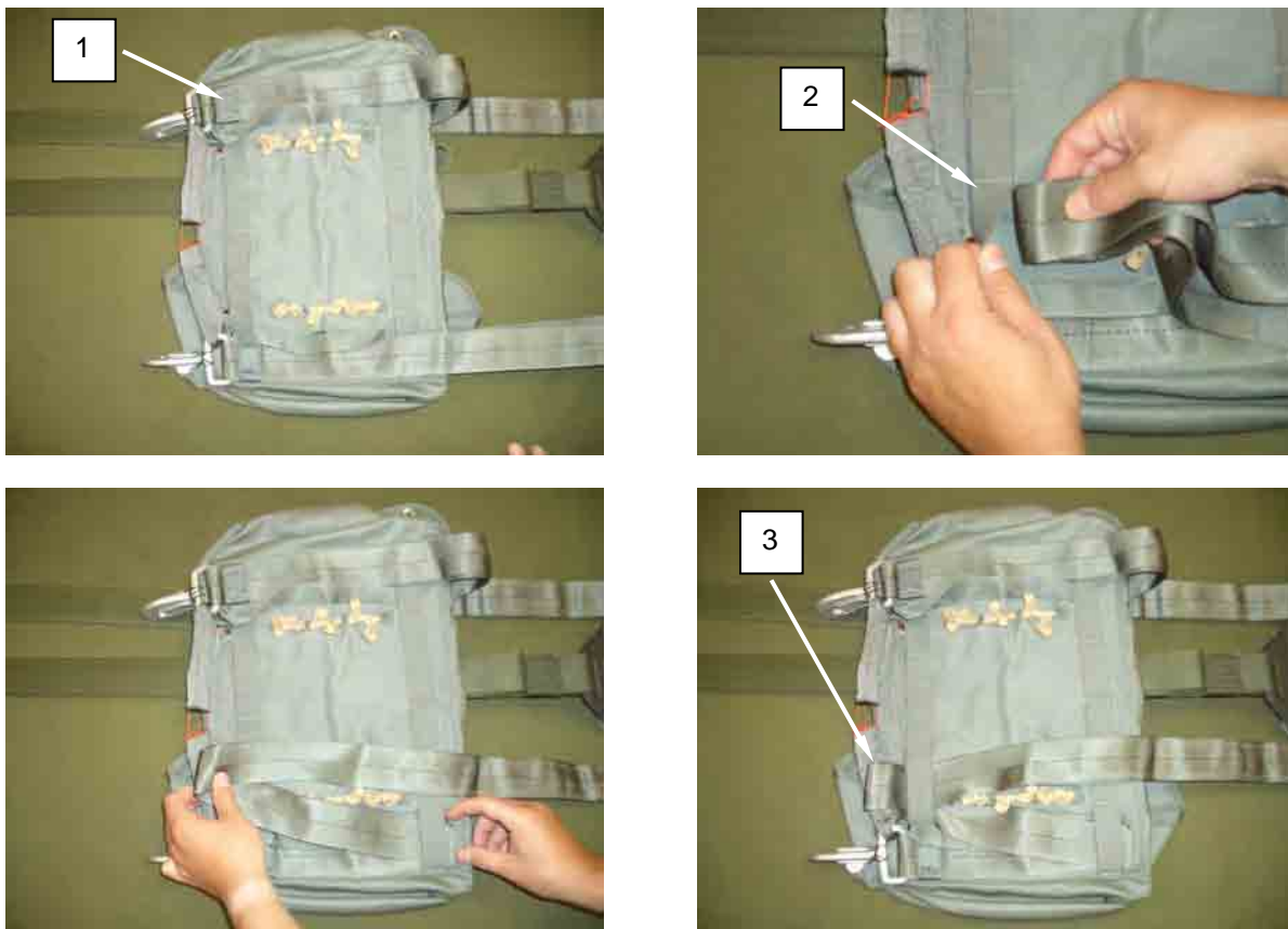
Figure 15. Partially S-Folding the Risers into Pack Tray.
