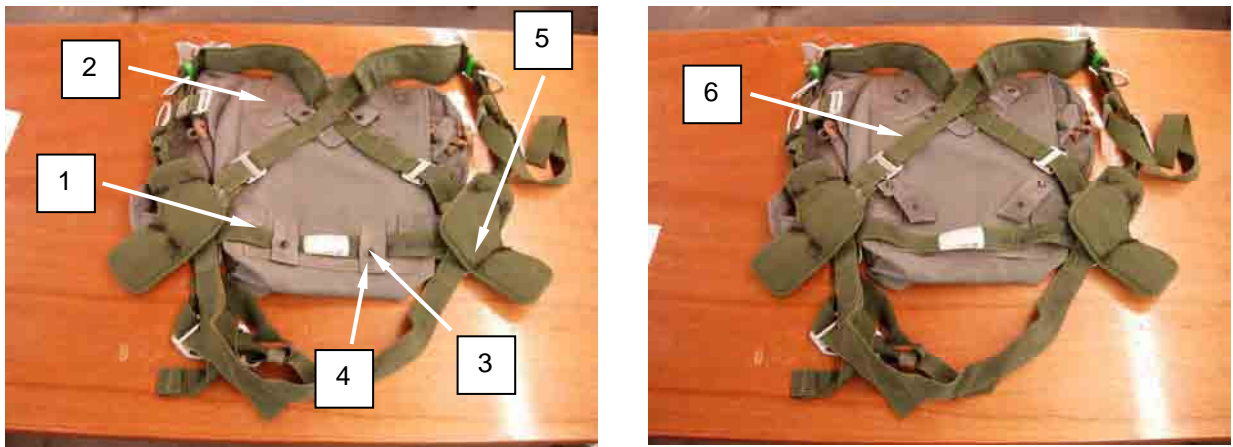
Figure 2. Removing Unserviceable Pack Tray.
