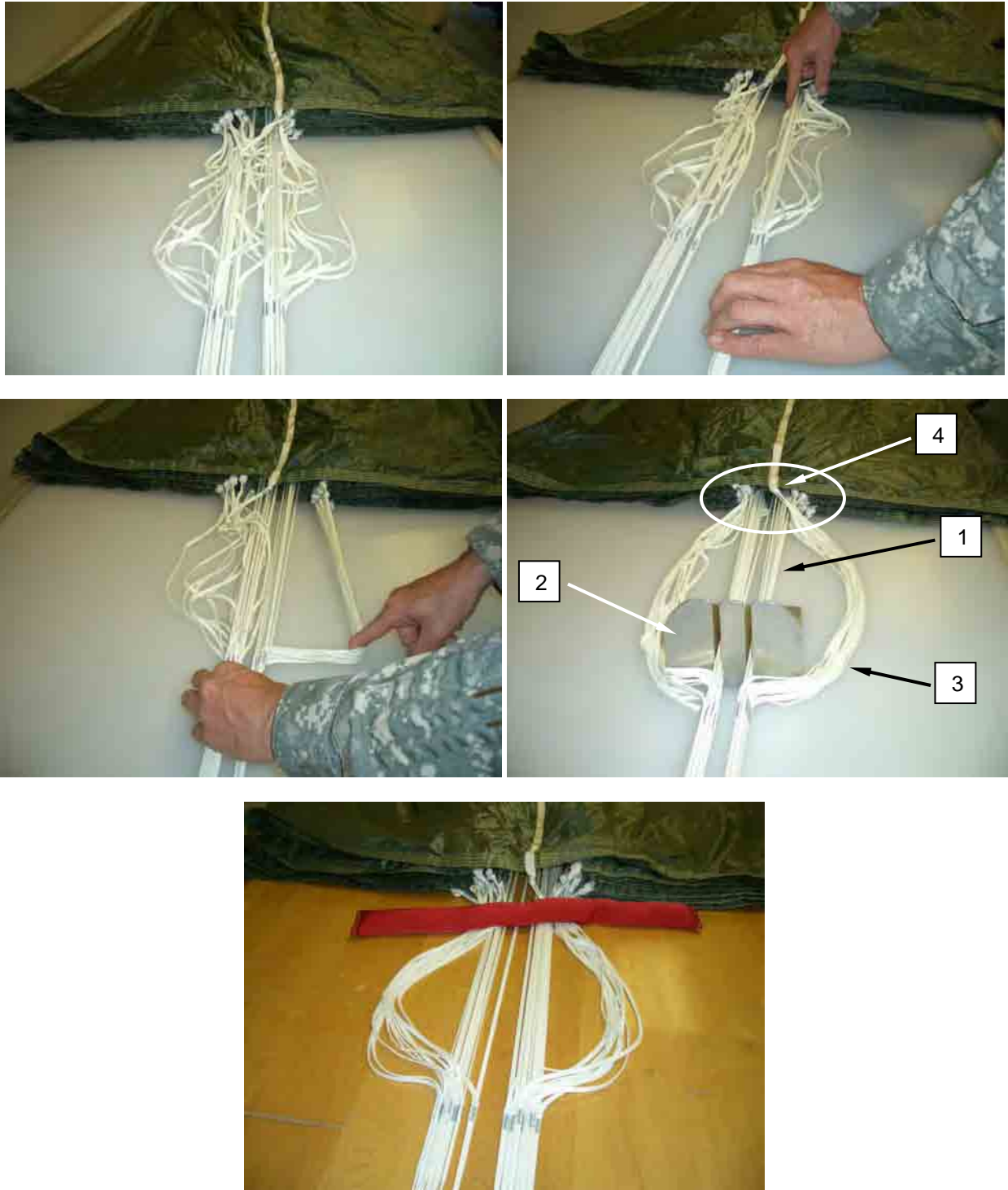
Figure 18. Organizing the Skirt Assist Lines Entering the Canopy.
