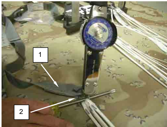
Figure 9. Tighten Barrel Nut on Connector Link.
