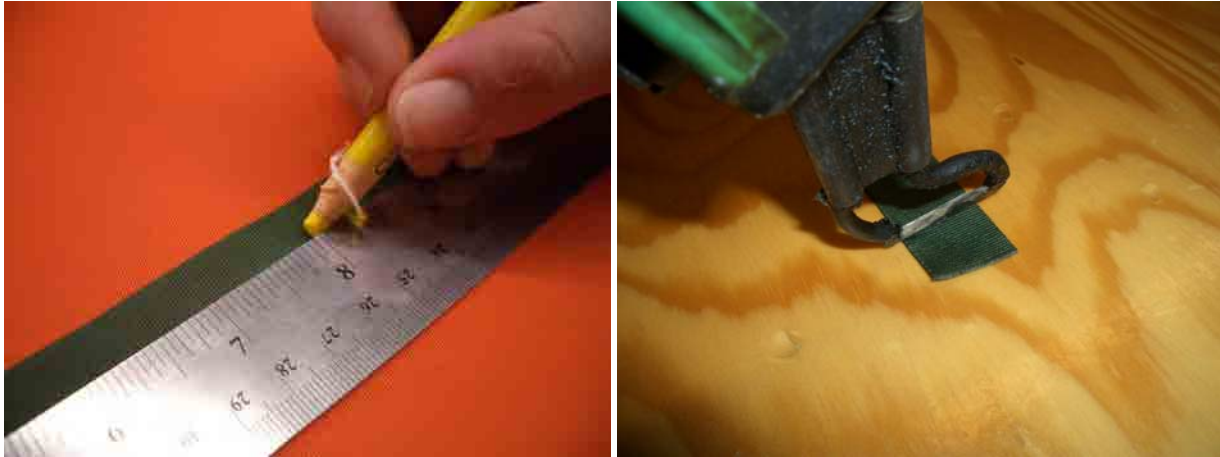
Figure 3. Cutting a 15½-inch Length of Type I Nylon Webbing.
