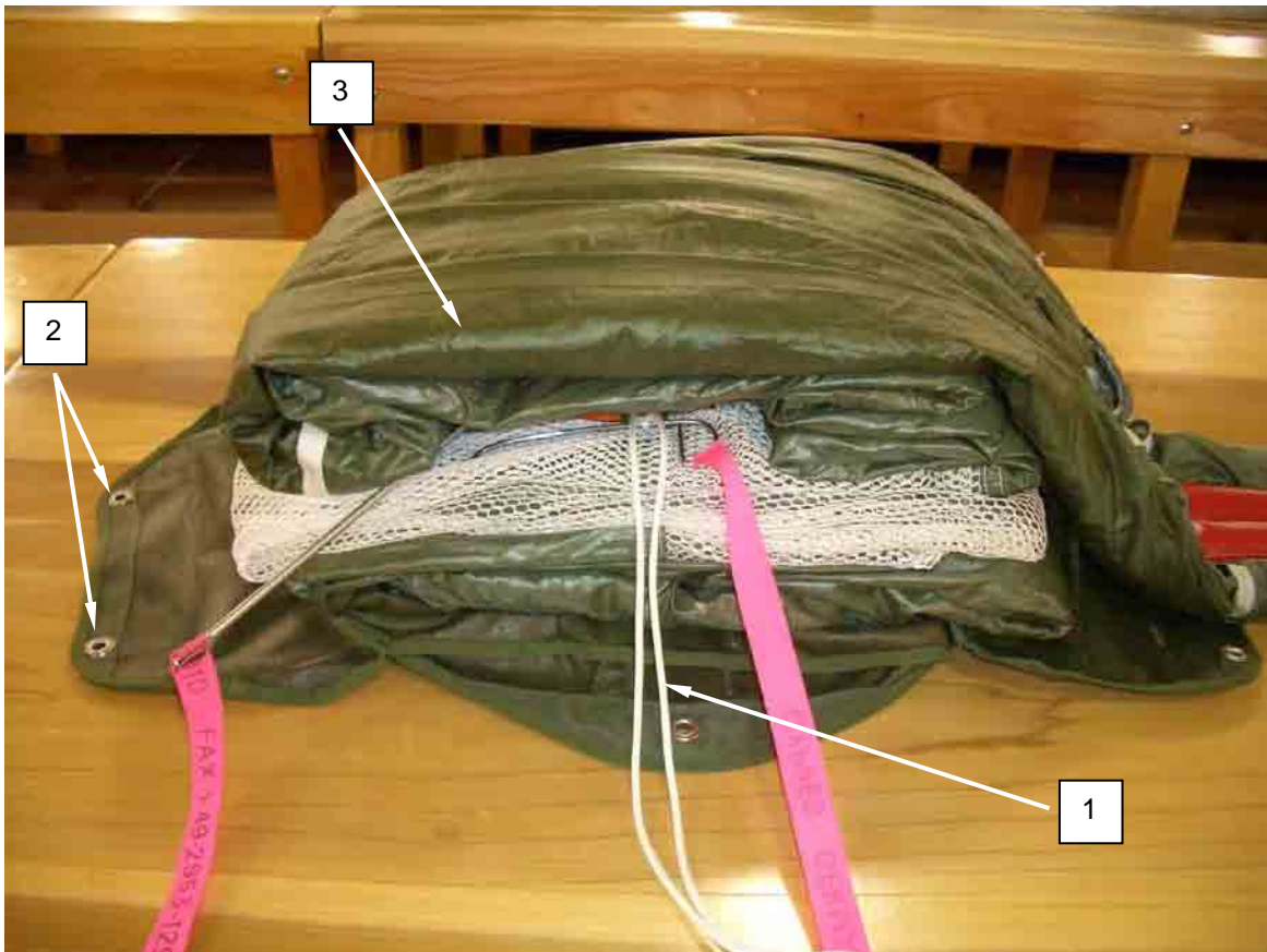
Figure 48. Forming a Bridge over Top of Ejector Spring.
