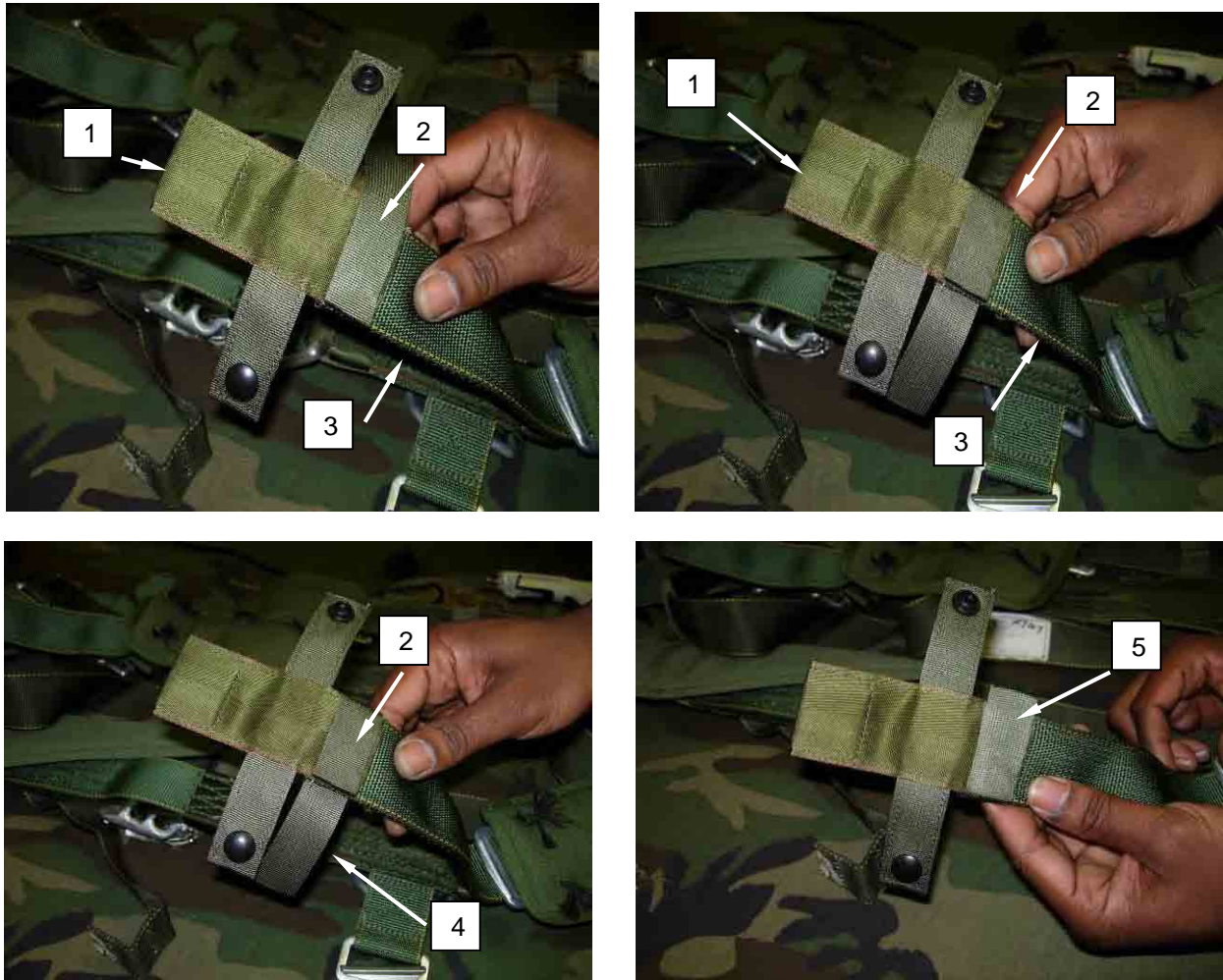
Figure 12. Attach Tuck Tab Assembly to the Upper Main Lift Web Assemblies.
