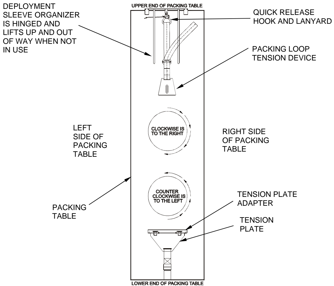
Figure 1. Rigger’s View.
