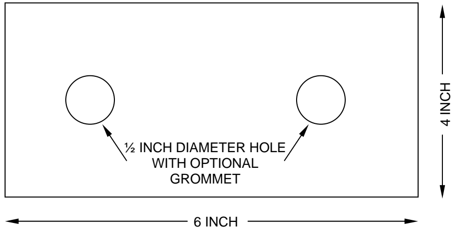
Figure 5. Reserve Ripcord Pull Handle Cuff.
