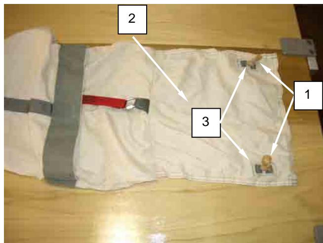
Figure 26. Attaching Retainer Bands to Deployment Sleeve Bridle Line Stow Panel.
