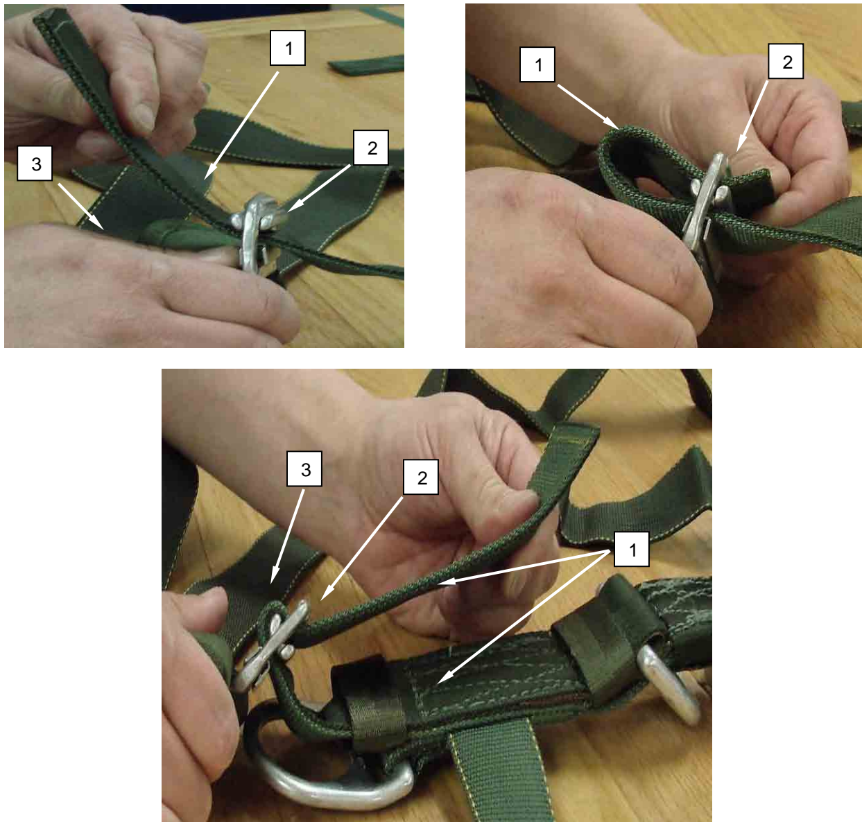
Figure 7. Routing of the Left Upper Main Lift Web Straps.
