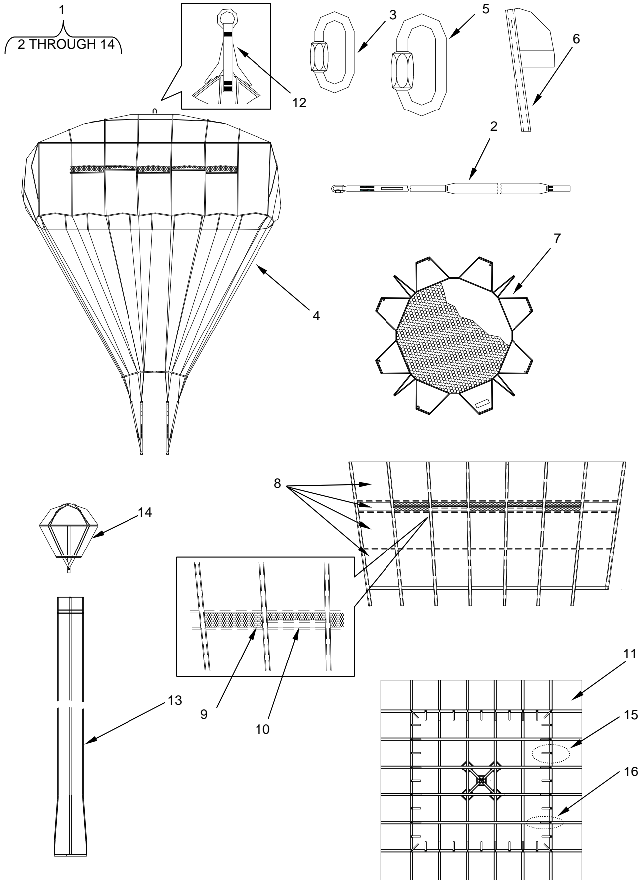
Figure 2. T-11 Main Parachute Assembly.
