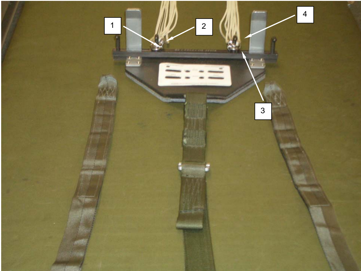
Figure 5. Riser Connector Links.
