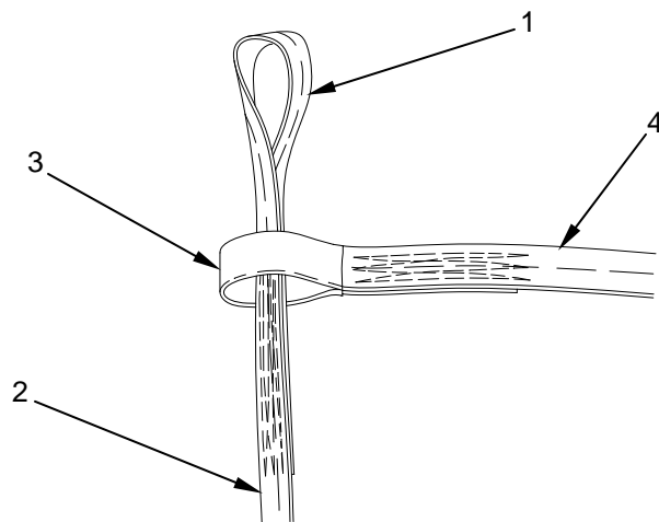
Figure 34. Passing Loop of Static Line through Buffer Loop on USL Extension.
