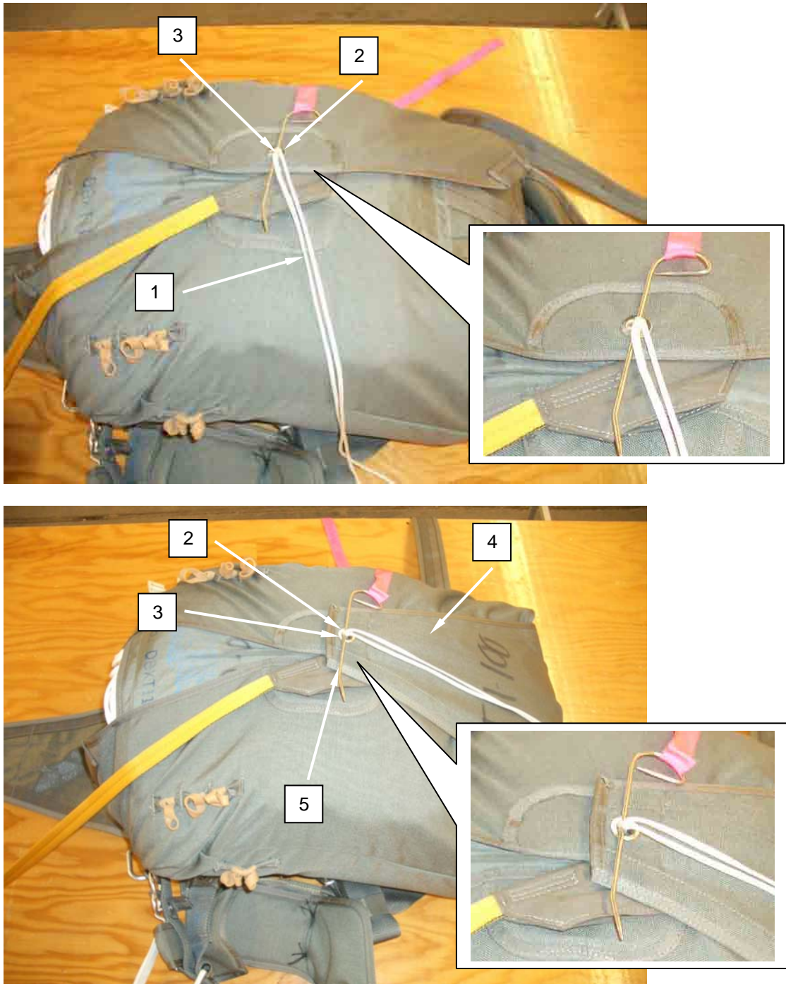
Figure 58. Close Bottom Flap and Secure with Temporary Pin.
