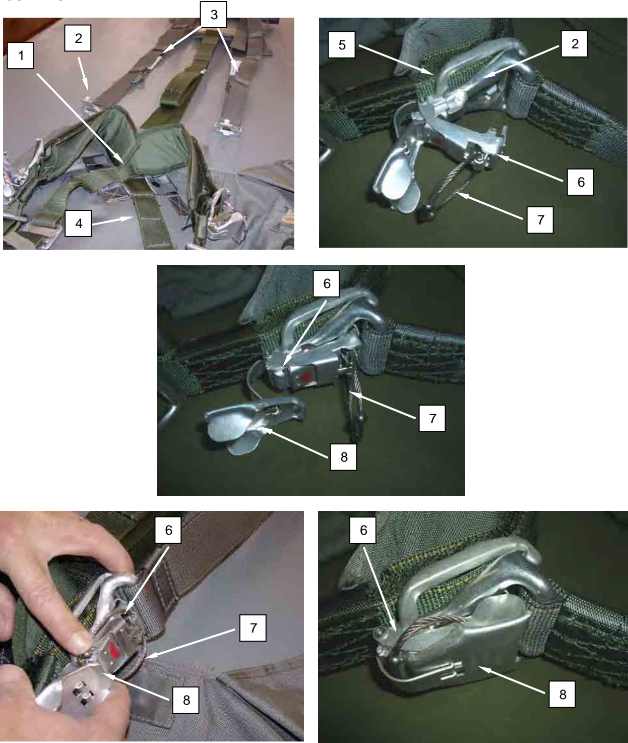
Figure 18. Laying Out Risers and Harness Assembly, and Assembling Risers and Harness Assembly.
