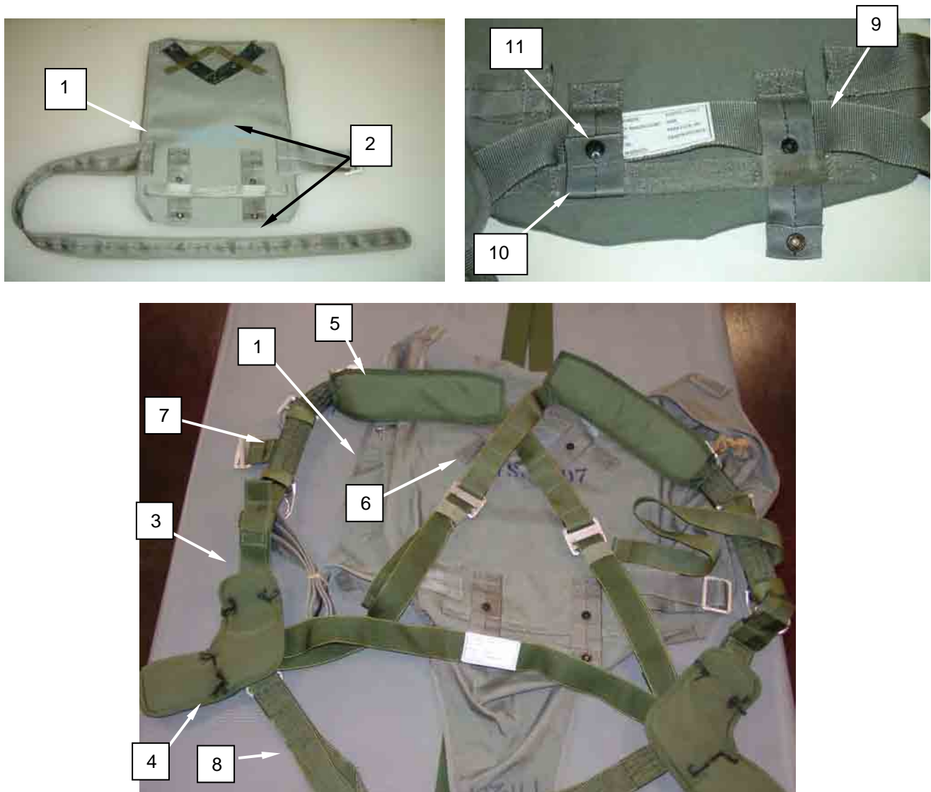
Figure 16. Pack Tray and Harness Assembly.
