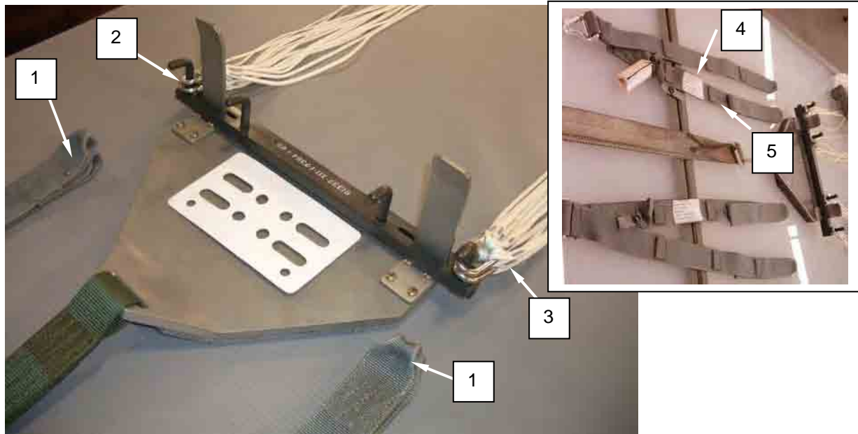
Figure 2. Lay Out Riser Assembly.
