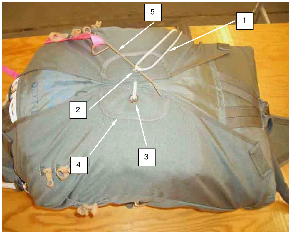
Figure 56. Close Side Flaps and Secure with Temporary Pin.
