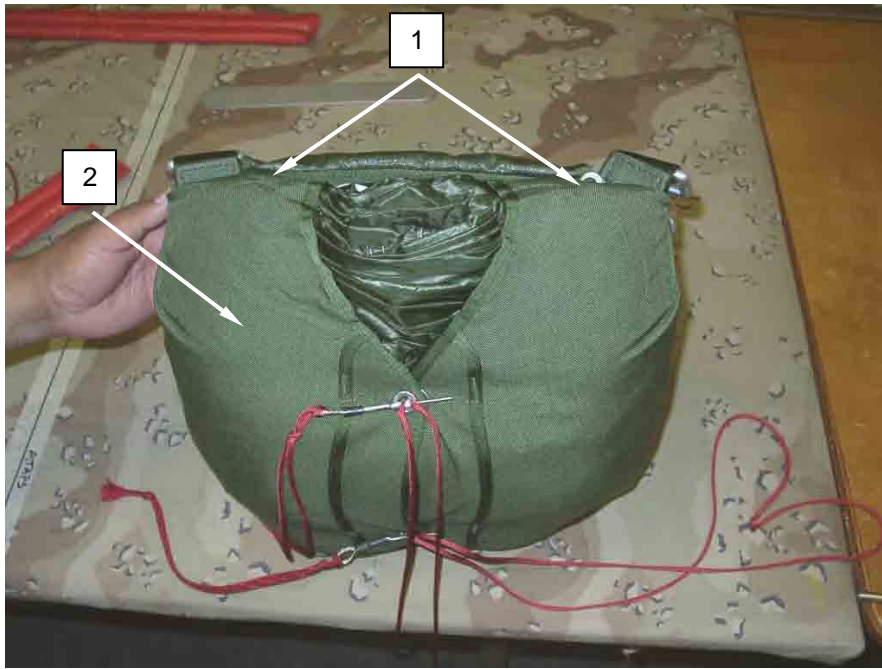
Figure 55. Tucking Left and Right Sides into Pack Tray.
