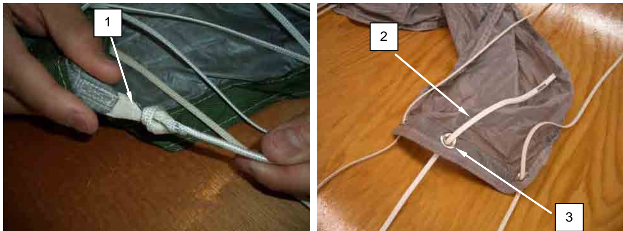
Figure 2. Routing Suspension Line through Slider.
