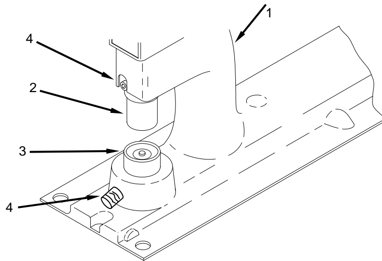
Figure 2. Hand or Foot Operated Press Method.
