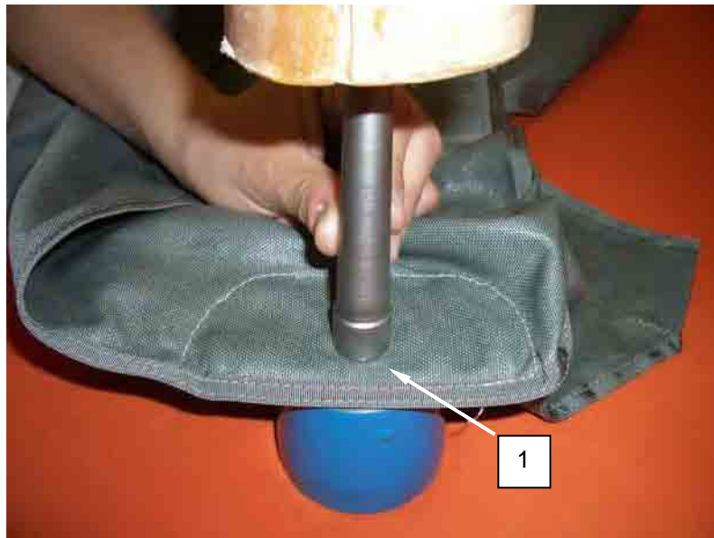
Figure 3. Spread Grommet Barrel.
