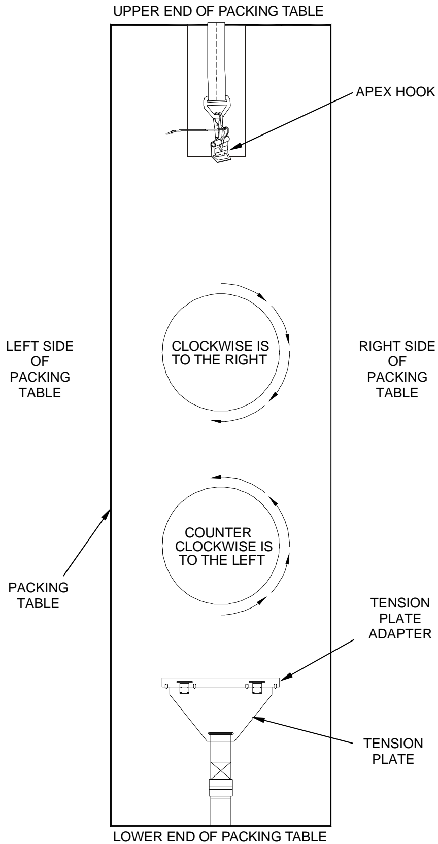
Figure 1. Rigger's View.
