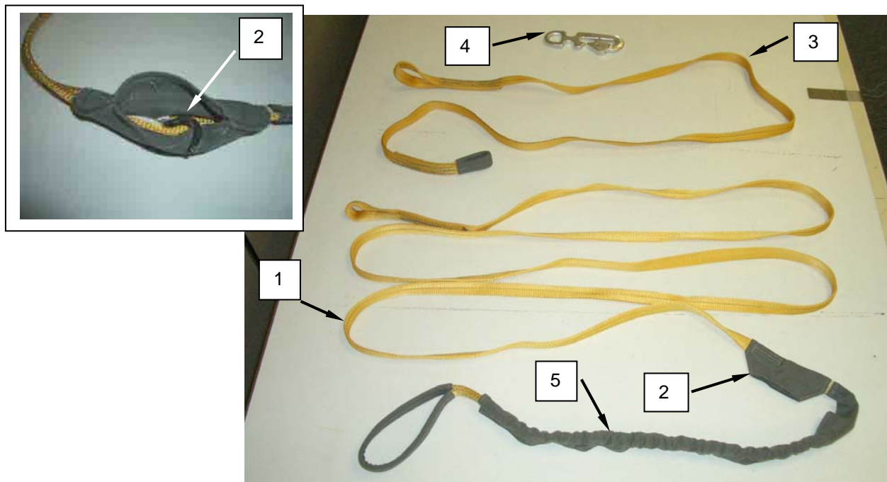
Figure 10. Universal Static Line Modified (with Curved Pin).
