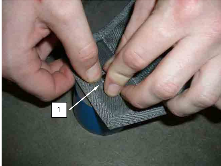
Figure 4. Insert Barrel of Replacement Grommet through Accommodating Hole in Material.
