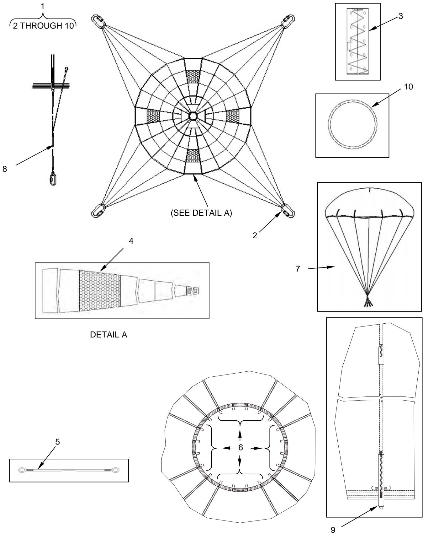
Figure 6. T-11R Canopy Assembly.
