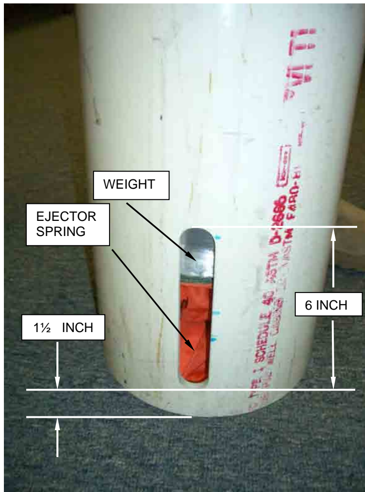
Figure 1. Spring Compression Test Tube.
