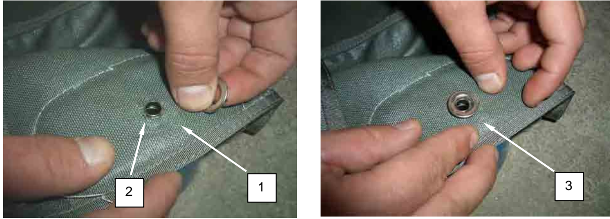
Figure 2. Insert Barrel of Replacement Grommet through Accommodating Hole.
