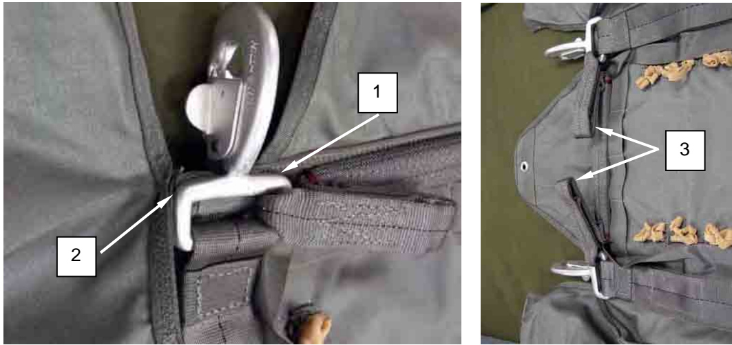
Figure 12. Aligning Top Bar of Snap Hook with Binding Tape and S-Folding Excess Spreader Bar.
