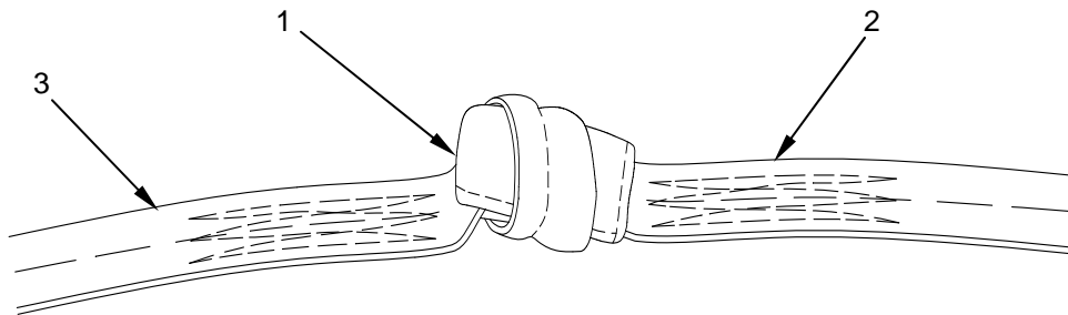
Figure 36. Making Girth Hitch Securing USL Extension to Static Line.
