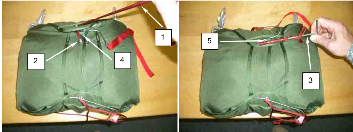
Figure 57. Inserting Second Temporary Pin.
