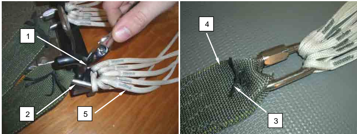
Figure 1. Removing Connector Links.
