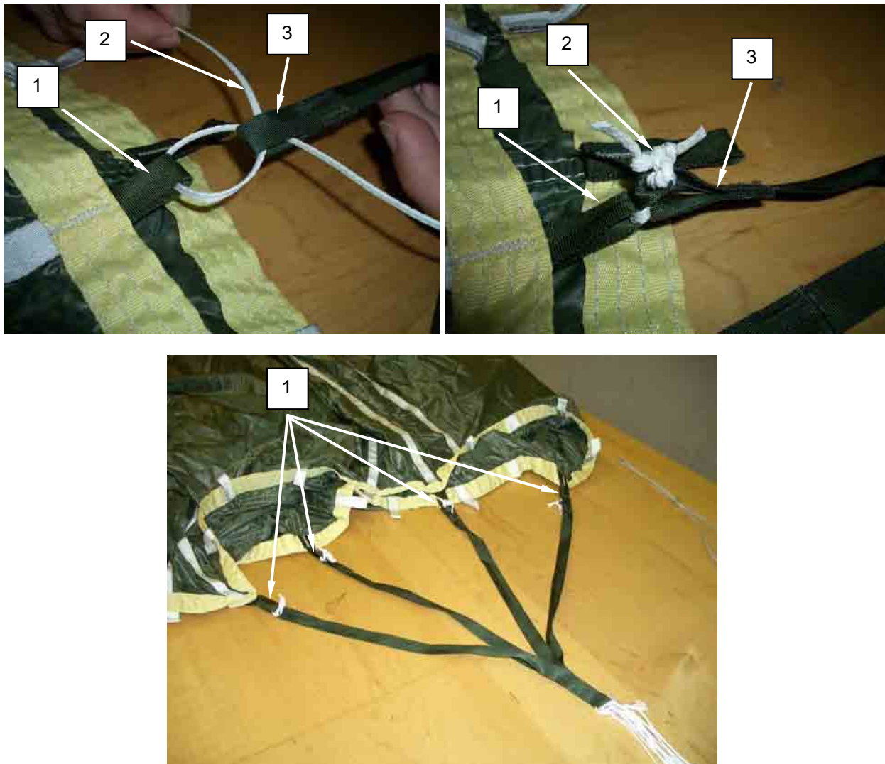
Figure 2. Attach Reserve Extractor Parachute.
