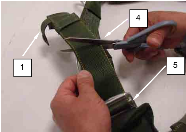
Figure 3. Replacing Harness Left Upper Main Lift Web Assemblies.
