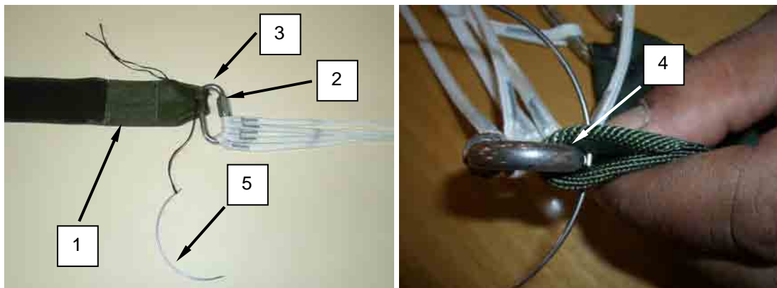
Figure 10. Tack Riser with Lacing and Tying Tape.
