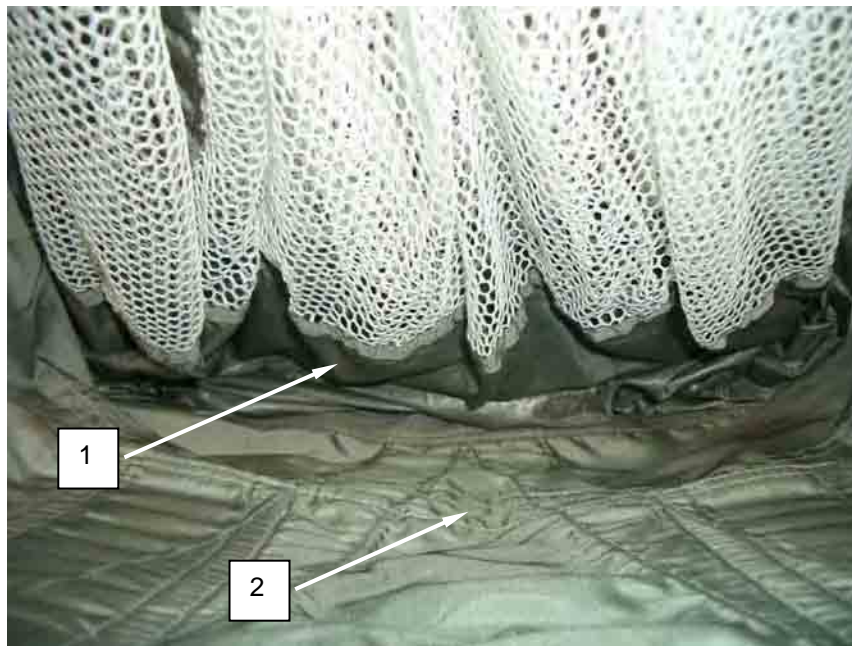
Figure 41. Place Drogue Parachute into Deployment Bag.
