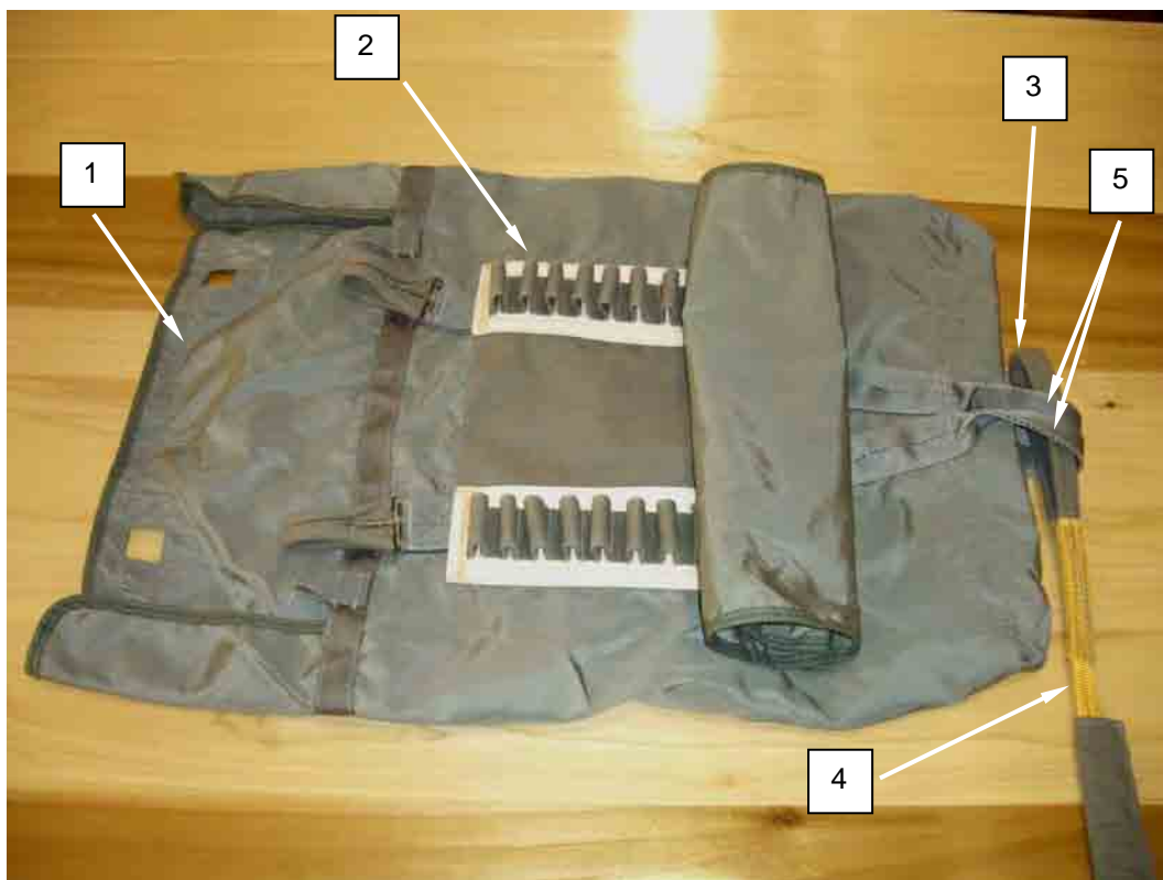
Figure 27. Passing the 6-inch Buffer Loop through Deployment Bag Reinforcement Webbing.
