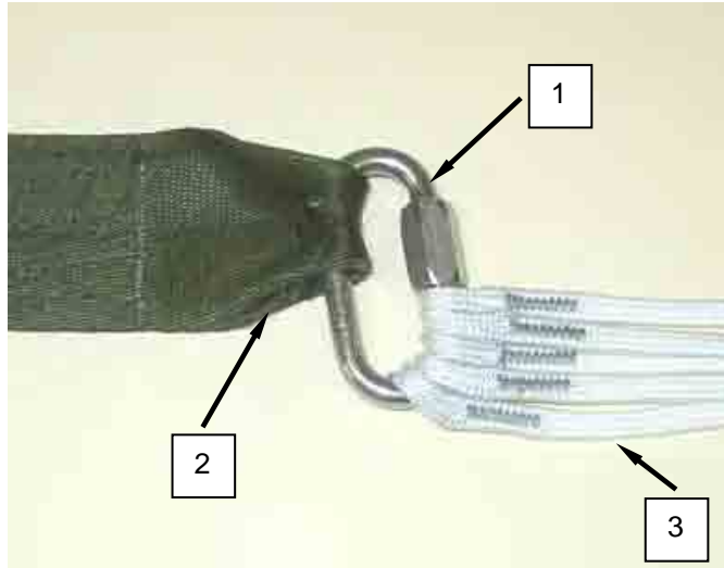
Figure 6. Rotate Connector Link to Riser.
