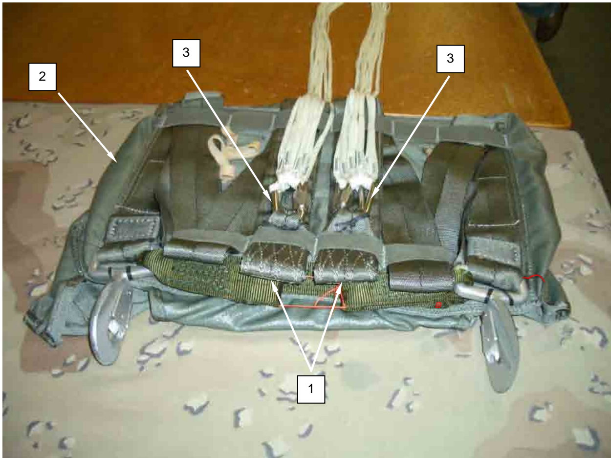
Figure 33. Making Two Remaining Riser Stows.
