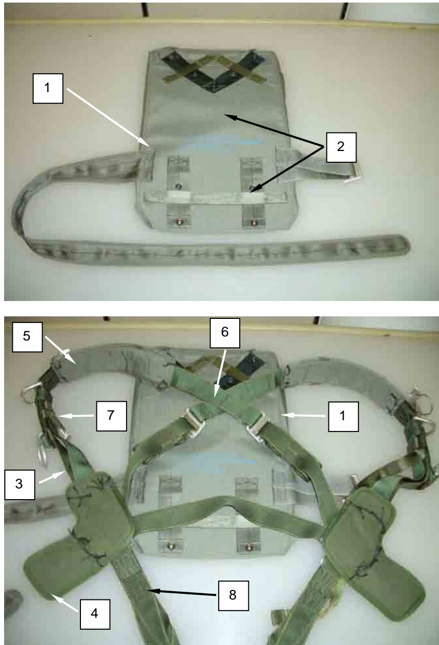
Figure 5. Pack Tray and Harness Assembly.
