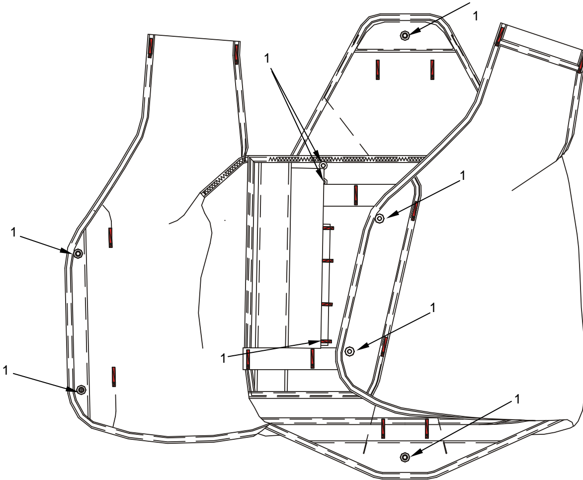
Figure 1. Reserve Pack Tray Grommet Size #0.
