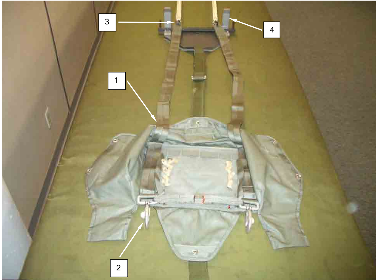
Figure 6. Placing Connector Links on Tension Plate Adapter.
