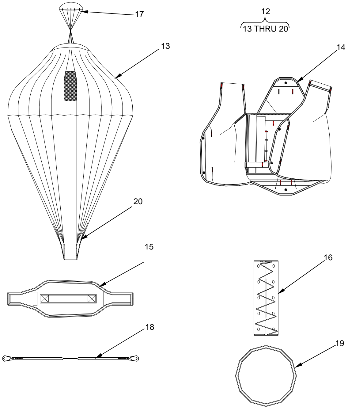
Figure 1. T-11 Personnel Parachute System (Sheet 2 of 2).
