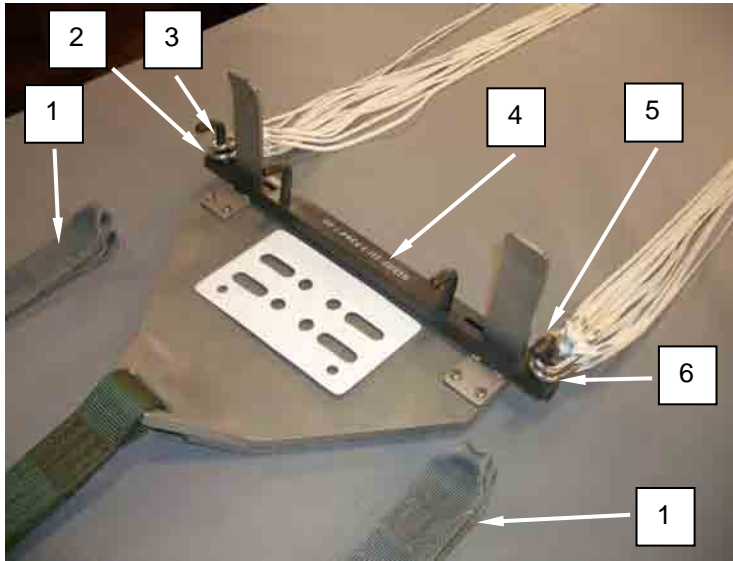
Figure 2. Lay Out Riser Assembly.
