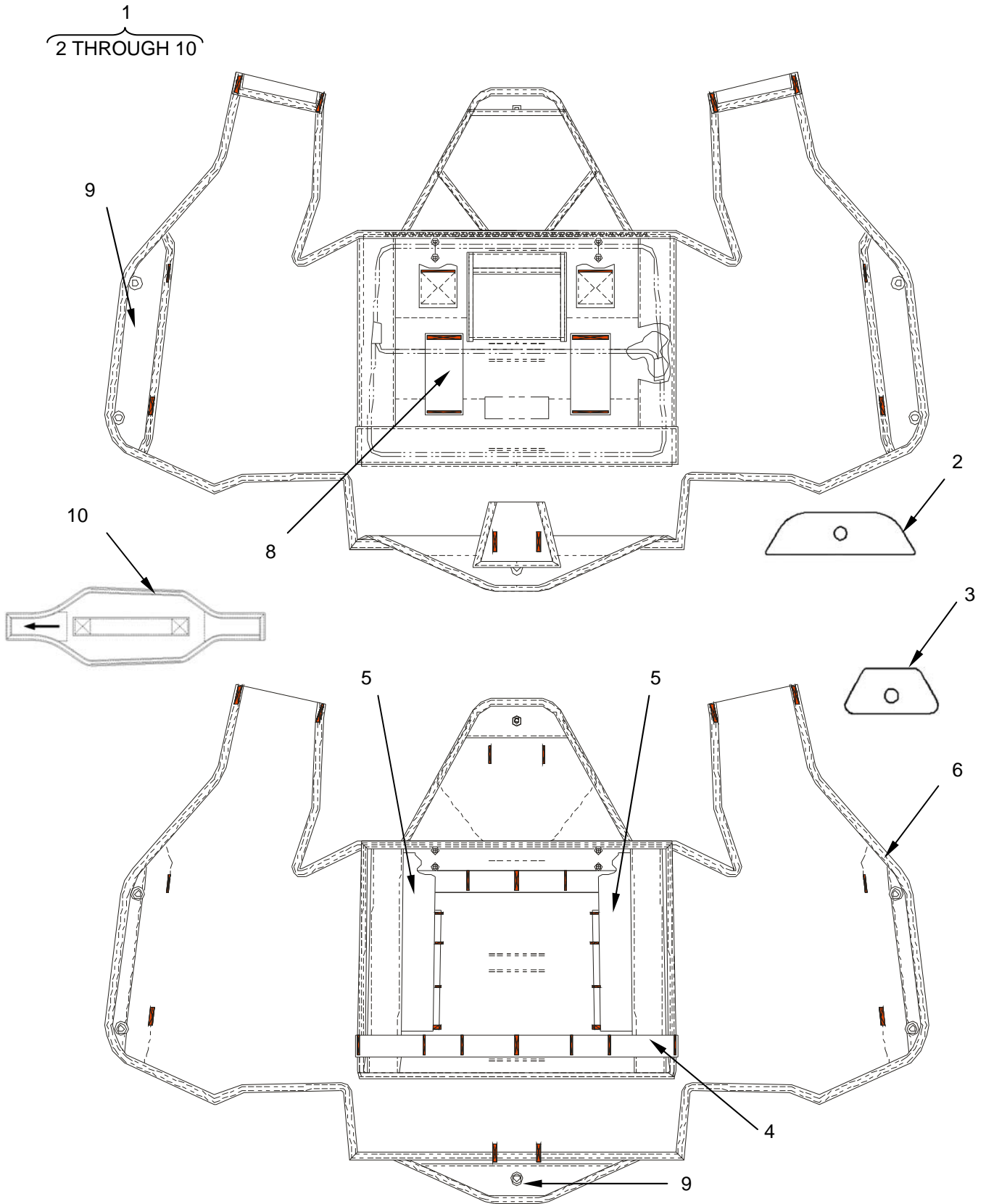
Figure 8. T-11R Pack Tray Assembly.
