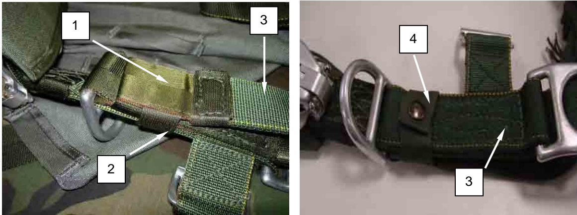
Figure 15. Secure Tuck Tab Assembly.
