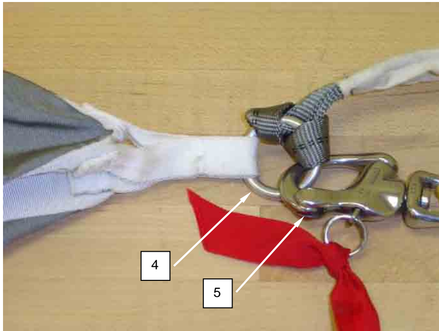
Figure 22. Attaching Bridle Ring to Quick Release Hook.
