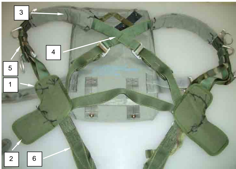
Figure 4. Pack Tray and Harness Assembly.
