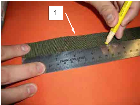
Figure 2. Cut New Tie-Down Loop Webbing.
