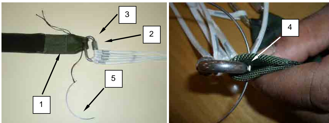
Figure 8. Tack Riser with Lacing and Tying Tape.
