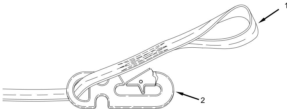
Figure 6. Pass the 3½-inch Loop End of Static Line through Opening of Snap Hook.
