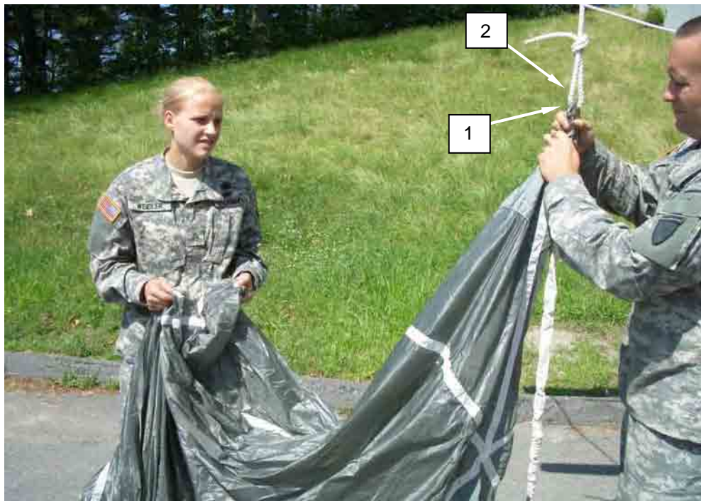
Figure 1. Connecting Snap on Pulley Rope to Canopy Bridle Loop.
